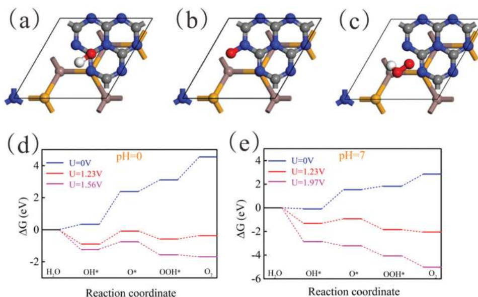
Fig. 10 (a)–(c) Optimized geometries of OH, O and OOH on the \text{In}_2\text{SeS/g-C}_3\text{N}_4 heterostructure during OER. (d) The changes of Gibbs free energy at pH = 0 and at different potential differences (0 V, 1.23 V and 1.56 V). (e) The changes of Gibbs free energy at pH = 7 and at different potential differences (0 V, 1.23 V and 1.97 V).
