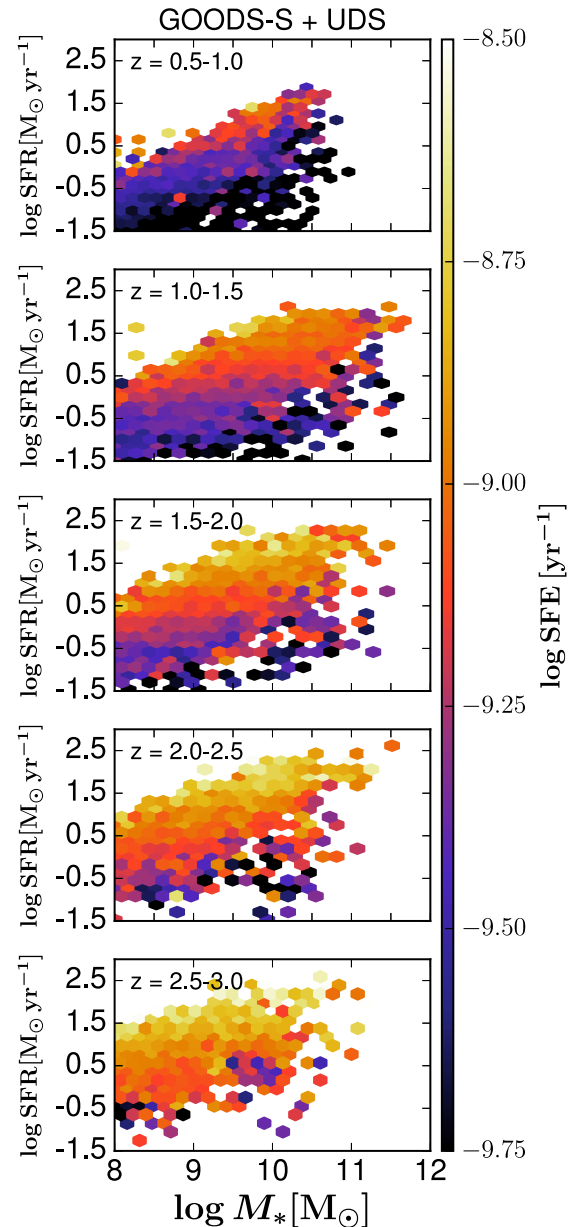
Figure 16. Galaxy SFR as a function of stellar mass for different redshift bins. The colour map gives the star formation efficiency ( \text{SFE} \equiv \text{SFR}/M_{\text{gas}} ) of the galaxies.
