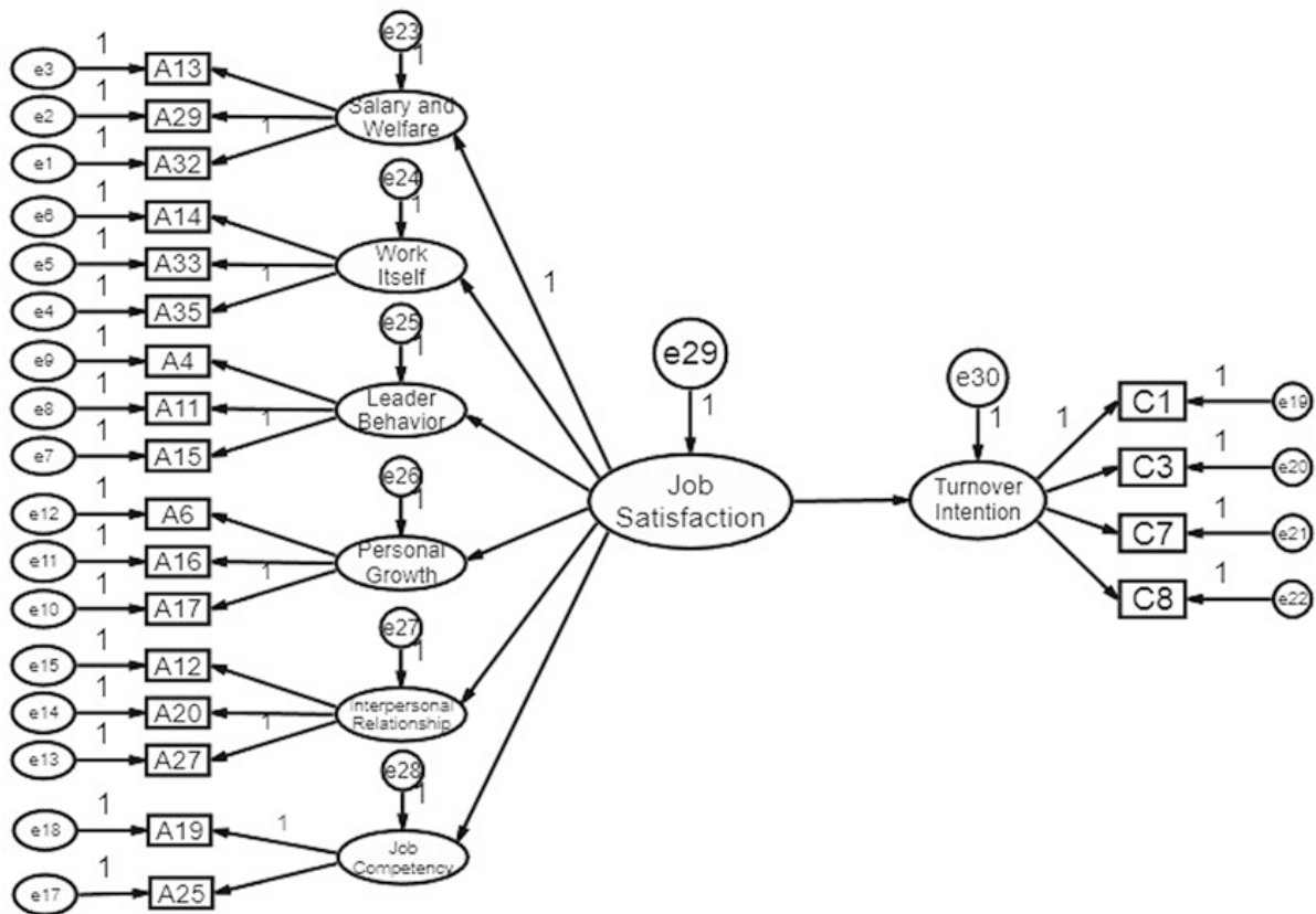
Figure 1. The structural equation model.
