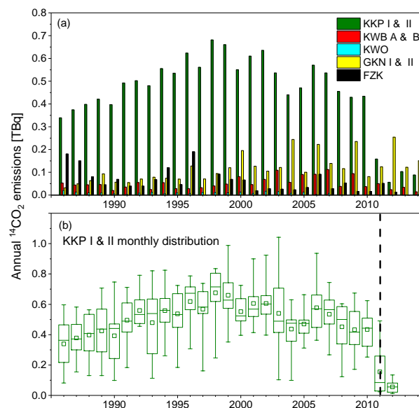
Figure 2. ^{14}\text{CO}_2 emissions from nuclear facilities: annual mean emissions from all facilities (a) and box plots of the distribution of monthly values from Philippsburg (KKP I and II, b); the boxes include 50 % of all months of the year with the horizontal bar indicating the mean and the square indicating the median value of the year. The whiskers show the minimum and maximum monthly values of the individual years. The dashed line indicates the shutdown of Philippsburg I shortly after the Fukushima accident.
