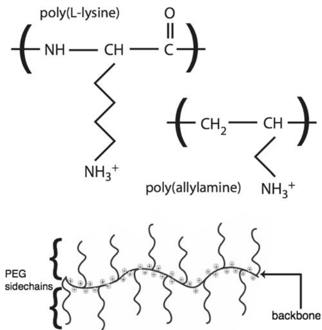
Fig. 1 Structure of poly(L-lysine) and poly(allylamine), and schematic structure of a brush-like graft copolymer with a polycationic backbone and a grafting ratio of 4
