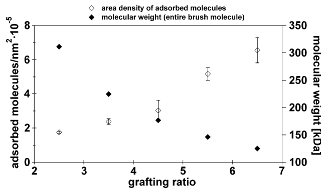
Fig 7 Number of molecules adsorbing per square nanometer and molecular weight of PAAm(14)- g -PEG(5)
