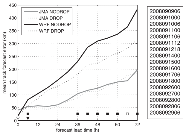
FIG. 6. Mean track forecast error of (gray) JMA and (black) WRF DROP and NODROP experiments. The track forecasts errors were averaged for 17 initial times displayed to the right of the figure and all verification times before 1200 UTC 20 Sep and 1200 UTC 30 Sep 2008, where forecasts from both models were available. Empty (filled) markers indicate times where the mean differences are significant at a 90% (95%) confidence level. Squares and triangles stand for WRF and JMA, respectively.
