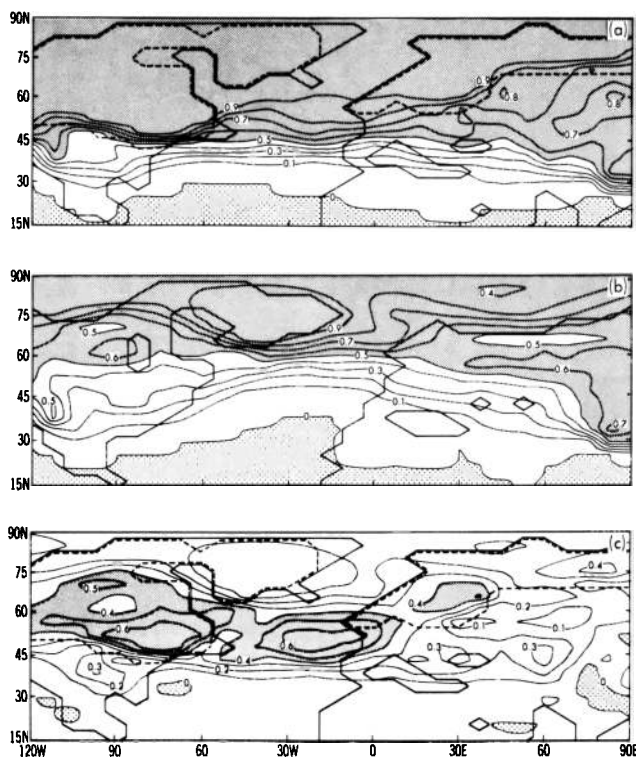
Fig. 30. Geographical distribution of (a) annual mean snow fraction (i.e., the fraction of precipitation falling as snow) obtained from the ice sheet experiment, (b) annual mean snow fraction obtained from the standard experiment, and (c) the difference between the two fractions (i.e., the ice sheet minus standard experiments). The dashed lines indicate the boundaries of the continental ice sheets.
