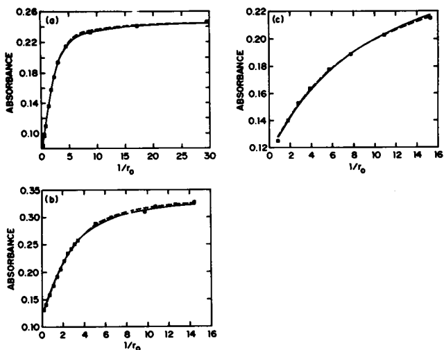
Figure 5. Absorbance at 442 nm of H 2 TMpyP/poly(dG-dC) solutions as a function of 1/r 0 at various sodium ion concentrations. In each case the best fit for the noncooperative model is shown by (—) while the overall best fit is shown by (- - - -). (a) [Na + ] = 0.03 M; ε f = 3.7 × 10 4 M -1 cm -1 ; ε b = 1.3 × 10 5 M -1 cm -1 ; K ω=1 = 1.01 × 10 6 M -1 ; ω = 0.75, K = 1.24 × 10 6 M -1 . (b) [Na + ] = 0.1 M; ε f = 4.4 × 10 4 M -1 cm -1 ; ε b = 1.18 × 10 5 M -1 cm -1 ; K ω=1 = 3.47 × 10 5 M -1 ; ω = 0.61, K = 4.32 × 10 5 M -1 . (c) [Na + ] = 0.3 M; ε f = 4.7 × 10 4 M -1 cm -1 ; ε b = 1.10 × 10 5 M -1 cm -1 ; K ω=1 = 5.96 × 10 4 M -1 ; ω = 1.9, K = 5.30 × 10 4 M -1 .
