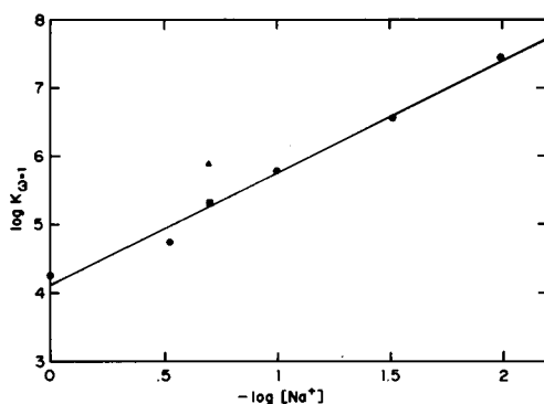
Figure 6. Plot of \log K_{0=1} vs -\log [Na^+] . The data of the present report is shown as (●). The results of the titration data of reference (9) are shown as (▲) while the value of K obtained from relaxation data (cf. reference 12) is shown as (■).
