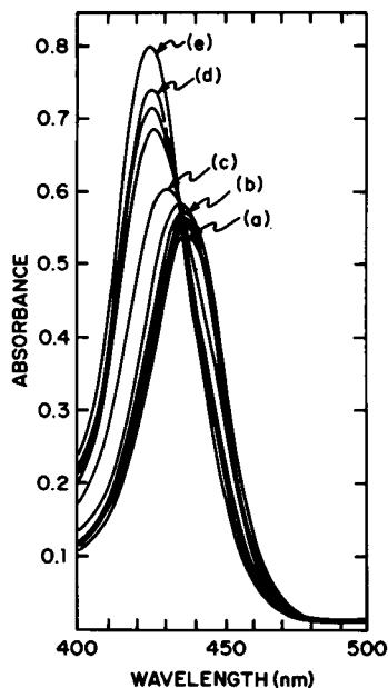
Figure 7. Absorbance of solutions containing 3.1 \mu\text{M H}_2\text{TMpyP} and 211 \mu\text{M} calf thymus DNA as a function of \mu . (a) \mu = .0040 \text{ M} , (b) \mu = .052 \text{ M} , (c) \mu = .50 \text{ M} , (d) \mu = 2.0 \text{ M} . Curve (e) is at the same conditions as curve (d) except no calf thymus DNA has been added.
