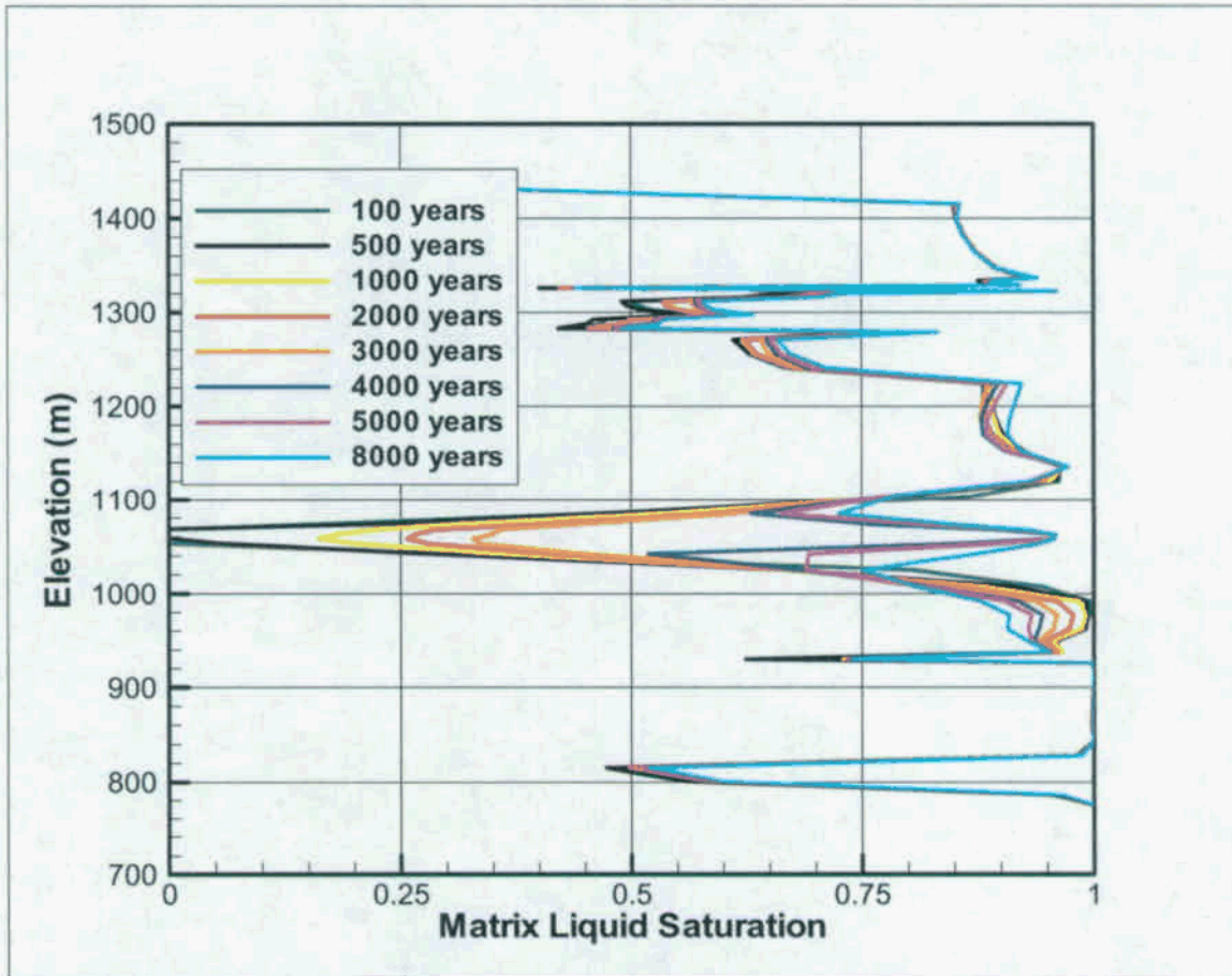
Figure 5a. Simulated matrix saturation along a vertical column from the ground surface to water table as predicted with thermo-ventilation model
