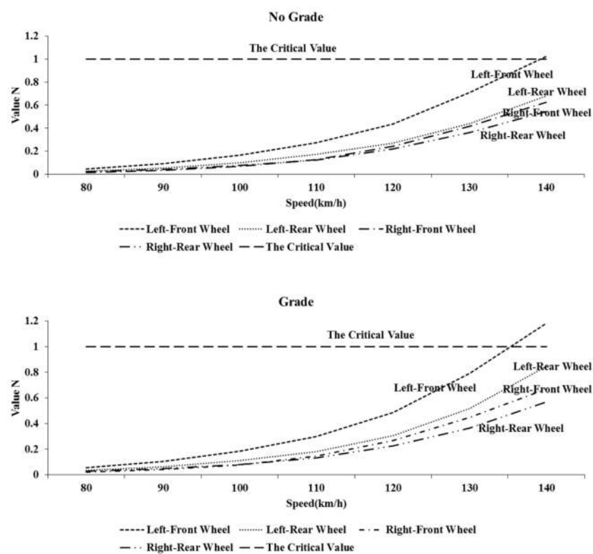
Figure 6. The critical skidding values of the SUV with or without grade.
