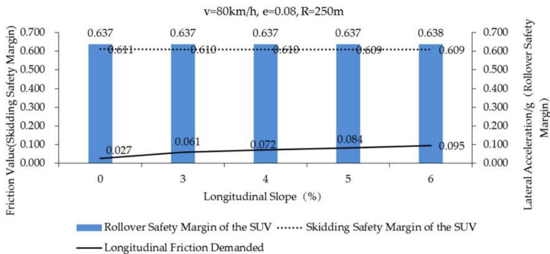
Figure 9. Skidding safety margin of the SUV, rollover safety margin of the SUV, longitudinal friction demanded of the SUV on good friction pavement ( f_{Tmax} = 0.85 ) (Case 7–11, in Table 5).
