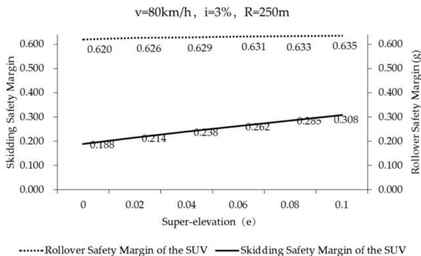
Figure 7. Friction demand of the SUV on good friction pavements.
