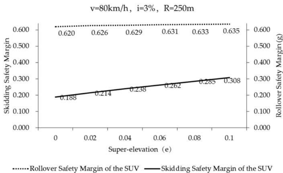
Figure 10. Skidding and rollover safety margin of the SUV on poor friction pavement ( f_{Tmax} = 0.50 ) (Case 1–6, in Table 5).
