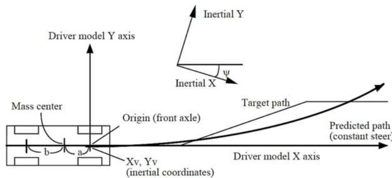
Figure 3. Axis system of steering controller.
