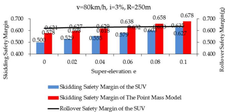
Figure 8. Skidding and safety rollover margin of vehicles on good friction pavement ( f_{Tmax} = 0.85 ) (Case 1–6, in Table 5).
