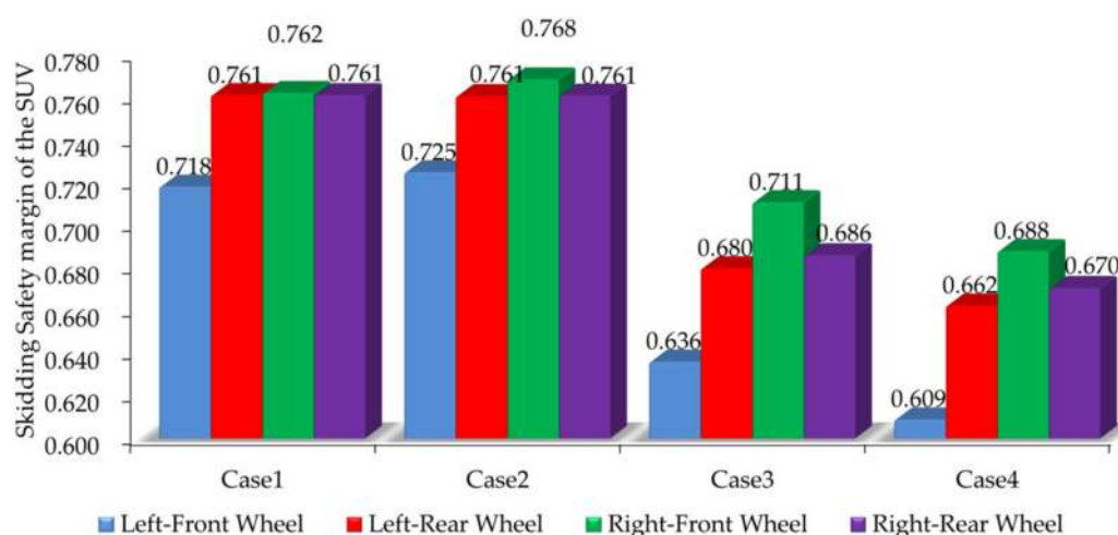
Figure 5. Skidding safety margins of four wheels under different road segments.
