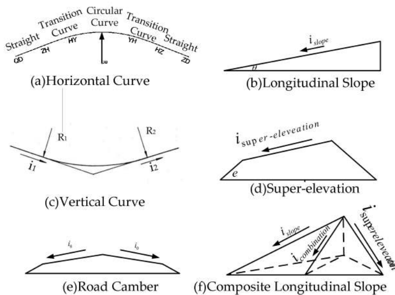
Figure 1. Road geometric parameters. (a) horizontal curve; (b) longitudinal slope; (c) vertical curve; (d) super-elevation; (e) road camber; (f) composite longitudinal slope.
