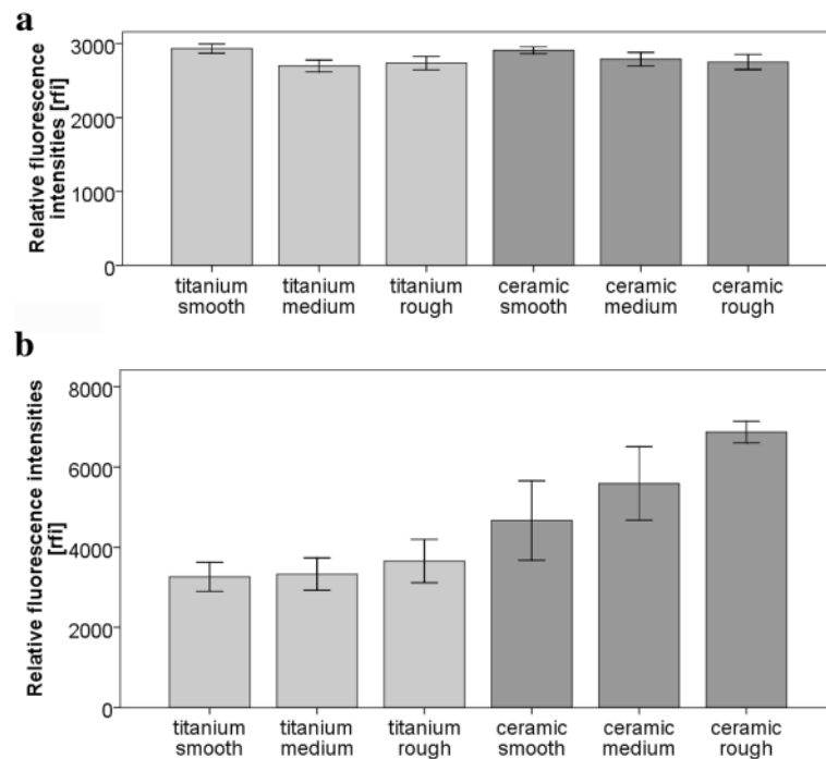
Fig. 3 Relative fluorescence intensities (rfi) of S. epidermidis (a) and S. sanguinis (b) on titanium and ceramic implant surfaces with different grades of roughness (means and standard deviations)
