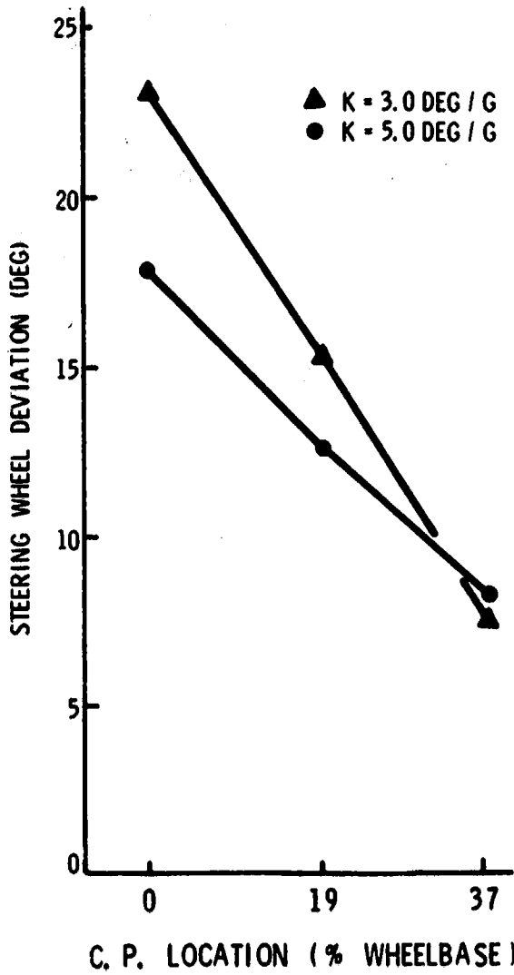
FIG. 9 COMBINED EFFECTS OF UNDERSTEER AND C.P. LOCATION AND OF CONTROL SENSITIVITY AND C.P. LOCATION ON STEERING WHEEL DEVIATION (RANDOM WIND GUST)
