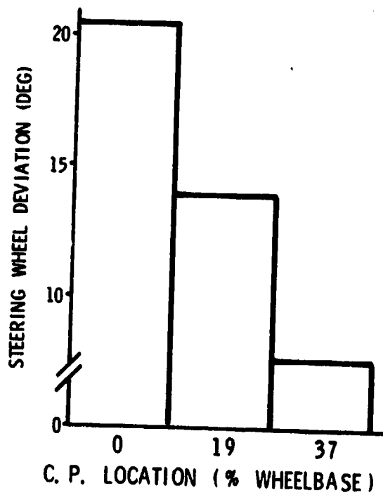
FIG. 8 EFFECTS OF UNDERSTEER, CONTROL SENSITIVITY, AND C.P. LOCATION ON STEERING WHEEL DEVIATION (RANDOM WIND GUST)
