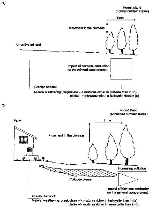
FIG. 1. Schematic representation of the impact of soil, saprolite and ground water pollution on the intensity of mineral weathering and on the rates of biomass production.
