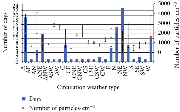
FIGURE 4: Number of particles registered and standard deviation for each Circulation Weather Type in 121 days in the months of June, July, August and September, in accordance with the days with each particular weather type.
