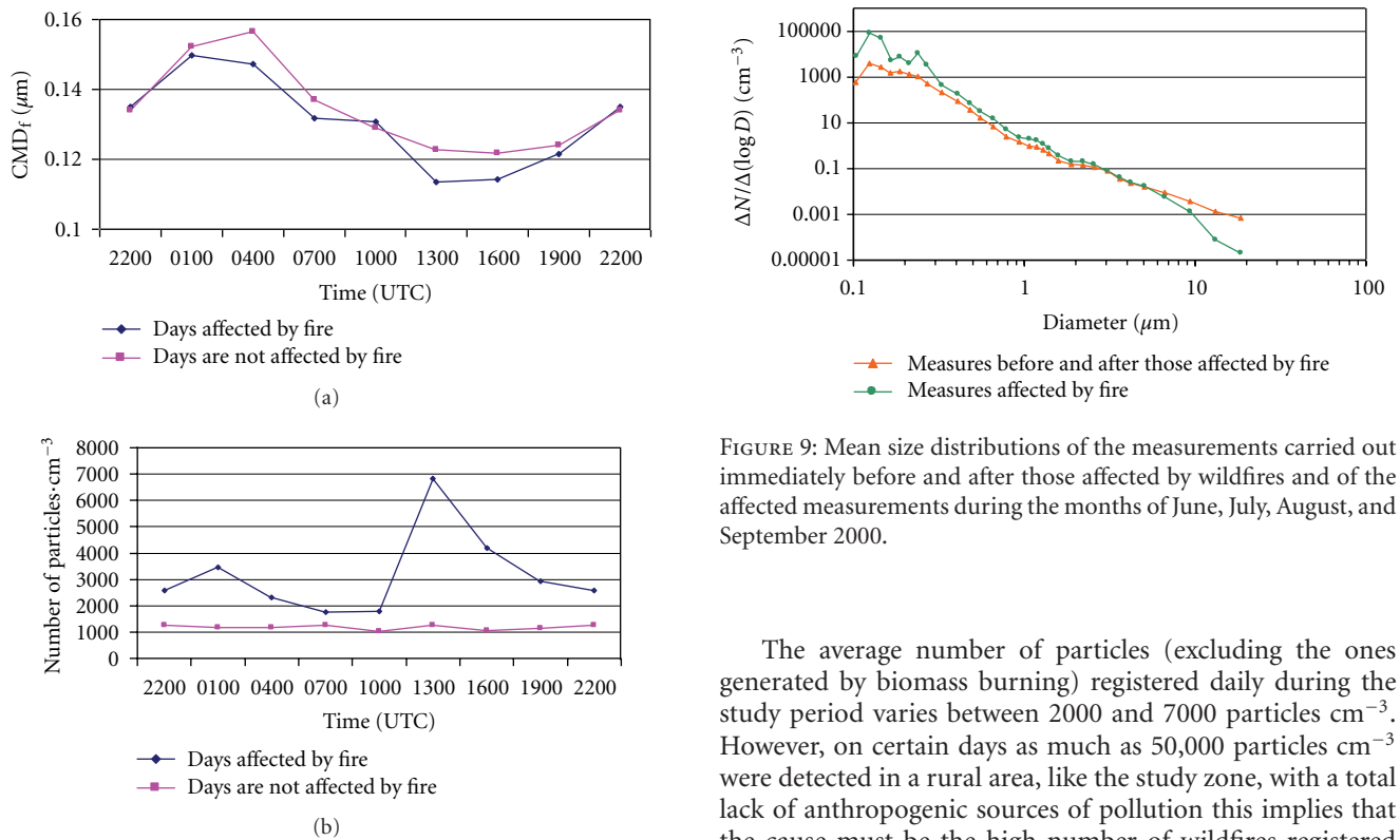
FIGURE 8: Comparative analysis of the evolution of (a) the geometric mean diameter (CMD f ) and (b) the total number of particles in the fine mode in the 8 daily registers, for data including contaminated and noncontaminated measurements.
