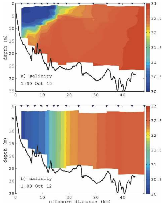
FIG. 9. Cross-shelf salinity sections on (a) 10 Oct, when winds were weak, and (b) 12 Oct, after the onset of strong downwelling winds (see Fig. 10). Station locations are indicated ( \blacktriangledown ) at the top of each section and the salinity color scale is shown to the right.
