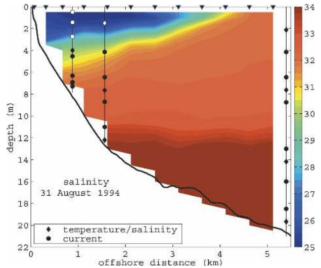
FIG. 4. Cross-shelf salinity section obtained from a small-boat survey ( \blacktriangledown indicate station locations) during a buoyant coastal current event on 31 Aug 1994. The vertical and cross-shelf location of instruments on the cross-shelf moored array are also shown. Salinity color scale is on the right.
