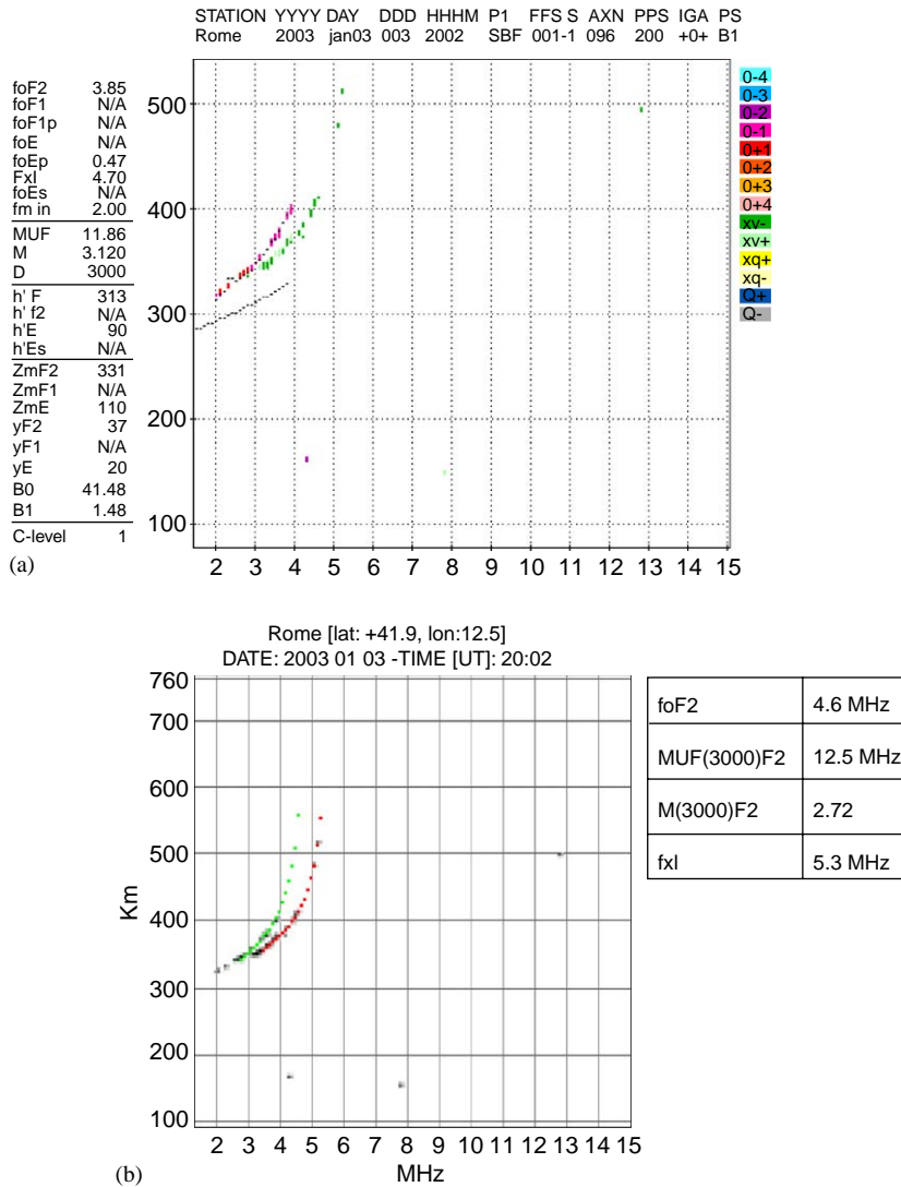
Fig. 3. (a) A case of truncated ionogram (subset T) for which ARTIST wrongly scaled foF2 as the last frequency recorded. (b) The same ionogram reported in Fig. 3a, with the trace correctly reconstructed by Autoscala. As output a reasonable extrapolated value for foF2 is given. The automatically reconstructed traces are reported (in green the ordinary trace and in red the extraordinary trace).
