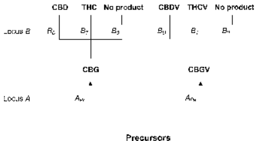
FIGURE 5.—The genetic model presented postulates the existence of two separate loci, A and B . Locus A has two different alleles A_{Pr} and A_{Pe} , responsible for the synthesis of either the propyl or the pentyl form of cannabigerol (CBG or CBGV, with R_1 = -C_3H_7 and R_2 = -C_5H_{11} ). Locus B has different alleles, each responsible for the conversion of CBG(V) into the end products CBD(V) and THC(V) accumulating in the inflorescences. The B_0 allele codes for a nonfunctional enzyme, leading to CBG(V) accumulation. All cannabinoids are drawn in their neutral form.
