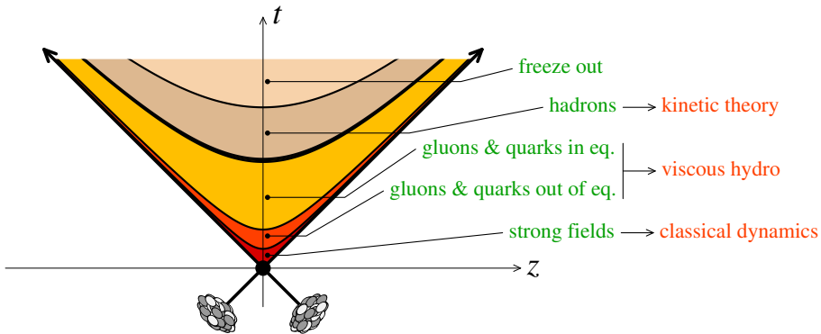
Fig. 5. Successive stages of a heavy ion collision.
