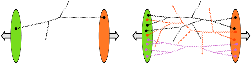
Fig. 9. Differences between a collision between dilute and dense projectiles.
