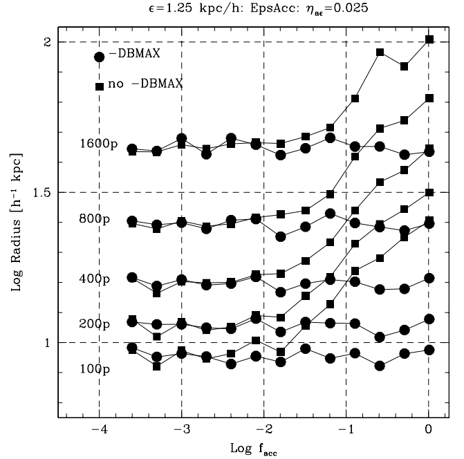
Figure 12. As Fig. 8, but for radii as a function of the GADGET force accuracy parameter, f_{\text{acc}} ( ErrTolForceAcc in GADGET ’s parameter file). The solid squares show results without enabling the extra-accuracy flag -DBMAX during compilation. The solid circles show results enabling -DBMAX . When this flag is on, the effects of f_{\text{acc}} on the mass are mild, and good convergence is achieved even for rather large values of f_{\text{acc}} . When -DBMAX is off, f_{\text{acc}} \lesssim 10^{-3} is needed to ensure convergence. This figure is in colour on Synergy , the online version of the journal.
