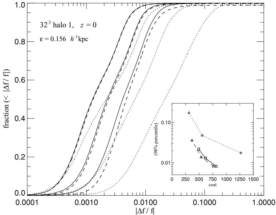
Figure 13. Cumulative error distributions of GADGET’s force computation for various choices of opening criterion and tolerance parameter. We used the particle distribution of a simulated CDM halo down to radii containing as few as 100 particles. Repeatability and robustness relative to these parameters are, of course, necessary conditions for convergence, but we must still demonstrate that the results do not depend on the total number of particles chosen. Figure 14. Shows a number of important trends. Consider, for example, the radius corresponding to 2 per cent of r_{200} (solid circles). In the 32^3 runs, this radius contains 1.6 per cent of the halo mass ( \sim 100 particles). The mass within this radius is seen to increase significantly as the number of particles increases; the density contrast climbs from \sim 1.2 \times 10^5 (in the 32^3 runs) to \sim 2.5 \times 10^5 (in the 64^3 runs) before stabilizing at \sim 3 \times 10^5 when N_{\text{sbox}} reaches 128^3 and 256^3 . Clearly, 100 particles are not enough to trace reliably the mass profile of a simulated halo, in disagreement with the conclusions of Klypin et al. (2001), who argue that 100–200 particles suffice to resolve the inner mass profile when other parameters are chosen properly.
