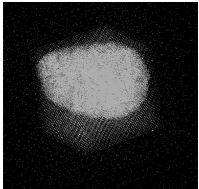
Figure 2. Particle distribution in the initial conditions of our 128^3 runs at z_i = 49 . Clearly seen is the ‘amoeba’-shaped region containing the highest-resolution particles, which is embedded within the 5.08 h^{-1} Mpc high-resolution cube used for the resimulation. Beyond the boundaries of the high-resolution cube lie massive particles that coarsely sample the entire volume of the 32.5 h^{-1} Mpc periodic box. This figure is in colour on Synergy , the online version of the journal.
