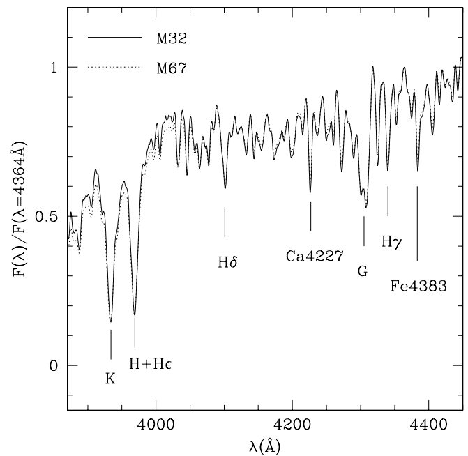
Fig. 8.—Comparison between the integrated spectra of M67 and M32. The spectra are very similar, although M32 looks to be slightly more strong-lined than M67, which suggests that M32 is on average slightly more metal-rich and younger than M67. See discussion in § 5.
