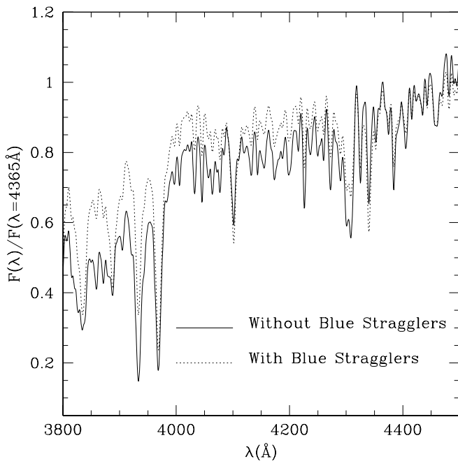
FIG. 4.—Integrated spectrum of M67, resulting from the computations described in § 3. The spectrum represented by the solid line was obtained without considering the contribution due to the BSs. The spectrum obtained when the latter are included is shown as the dotted line. The contribution due to the BSs is very large. This is a robust result, since the number of BSs relative to MS stars is solidly constrained by photometry and membership studies.
