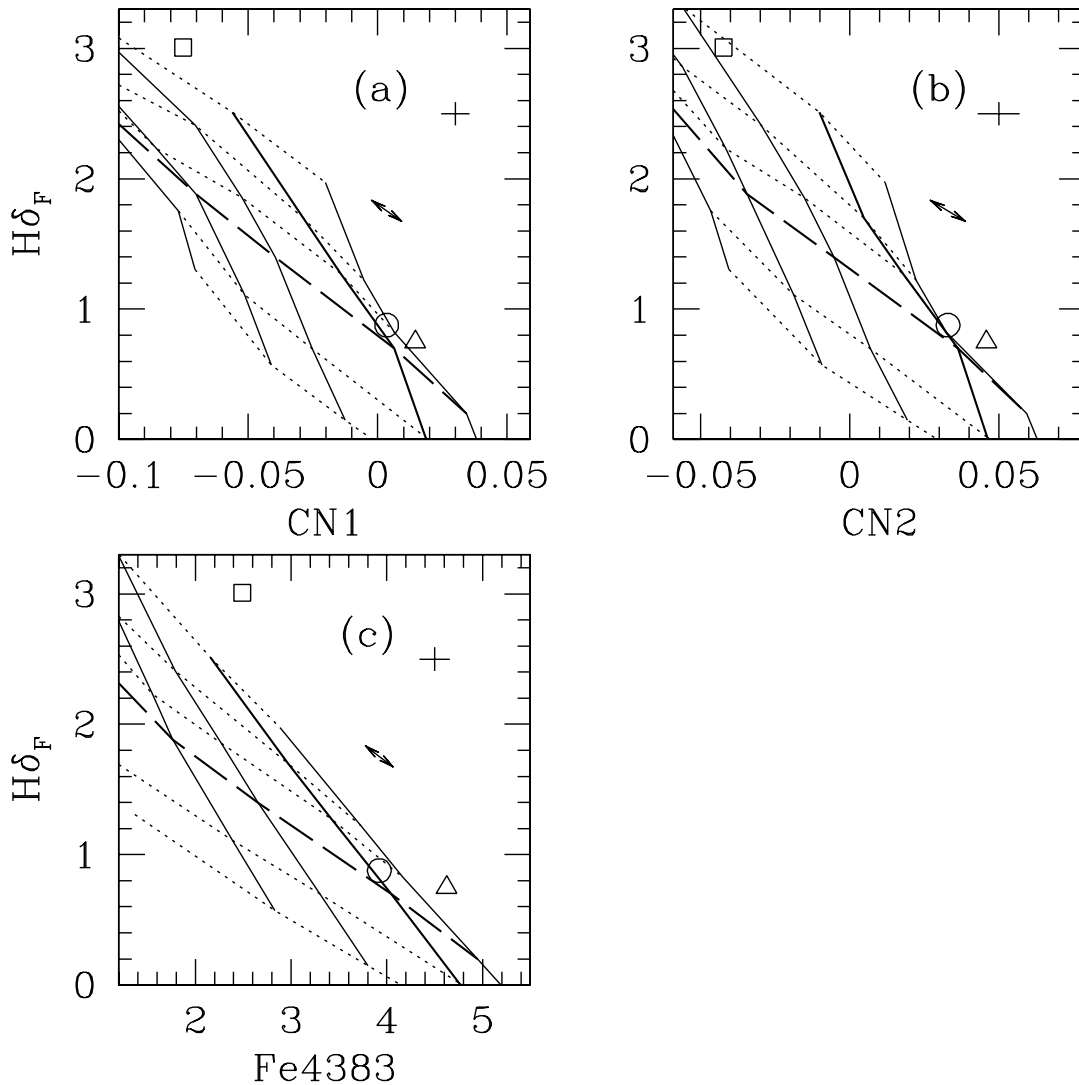
FIG. 6.—Comparison of model predictions absorption line indices for single stellar populations with those measured in the spectra of M32 (open triangle), M67 without BSs (open circle) and M67 including BSs (open square). Dotted lines connect model predictions for the same age. From top to bottom: 1.2, 2.0, 2.5, 3.5, 7.9, and 14.1 Gyr. Solid lines connect model predictions for the same [Fe/H] . From right to left: +0.2, 0.0, -0.4, -0.7, and -1.3 (in [c], the line for [Fe/H] = -1.3 falls outside the plotting area). The lines for [Fe/H] = 0.0 and age = 3.5 Gyr are thicker, for clarity. The arrows indicate by how much the integrated indices of M67 vary for an error of \pm 0.015 in E(B-V) . A higher reddening makes Balmer lines look stronger and metal lines weaker. The spectroscopic age of M67, when BSs are not included in the integrates spectrum, is about 3.5 Gyr in all diagrams, which is in agreement with the value inferred from the CMD. The data on M32 indicate that it has supersolar iron abundance and has a nearly solar abundance of carbon and/or nitrogen relative to iron.
