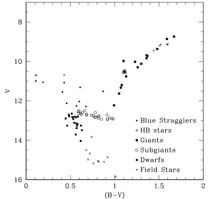
FIG. 1.—CMD showing the M67 members and field stars observed in this work. The photometry of M67 stars was taken from MMJ. Our observations of M67 members cover all the evolutionary stages of relevance for integrated light studies in the optical. Different evolutionary stages are denoted by different symbols, indicated in the bottom right corner. For completeness, we also observed field stars in areas where the CMD of M67 is scarcely populated (M giants) or where the stars are too faint to be observed efficiently (K dwarfs). Photometry of field stars was taken from the SIMBAD database, together with their Hipparcos parallaxes. The latter data were used to estimate the stars' positions in the CMD as if they were at the distance of M67.
