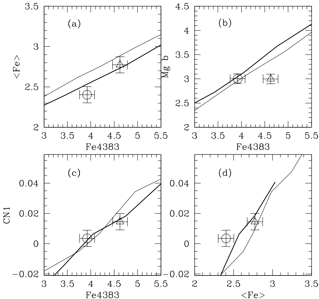
FIG. 9.—Data on M67 and M32 compared with single SP models on plots involving only abundance-sensitive indices. The symbols adopted are the same as in Fig. 6. Such plots are useful to unveil nonsolar-abundance ratios. Again, the open triangle and circle represent M67 and M32, respectively. The model lines are for [\text{Fe}/\text{H}] = 0.0 and +0.2 . The former is represented by a thick line. The lines connecting same-age models are omitted for clarity. While M67 is basically consistent with solar in all abundance ratios, M32 appears to have [\text{Mg}/\text{Fe}] substantially below solar. The combined abundances of C and N appear to be nearly solar in the center of M32.
