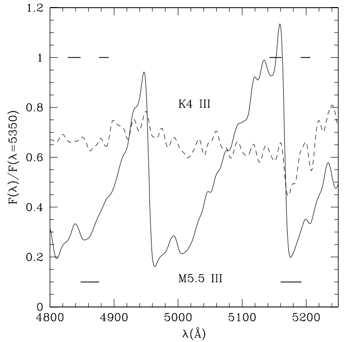
FIG. 3.—Comparison between the spectra of two giants: HD 94705 (M5.5 III, solid line) and HD 62721 (K4 III, dashed line), with essentially identical B-V values. The pseudocontinua and passband of H\beta (left) and Mg\ b (right) are illustrated by the horizontal lines. The spectrum of the M giant is characterized by very strong TiO bands, whose band heads coincide with the passbands and continuum windows of the Lick indices. The case of Mg\ b is particularly sensitive, since M giant stars contribute roughly 6 times more flux in the blue pseudocontinuum than in the index passband. For this reason, errors in estimating the contribution of very cool stars to the integrated light of M67 can cause sizable errors in the integrated value of Mg\ b . The same comments apply, to a lesser extent, to H\beta .
