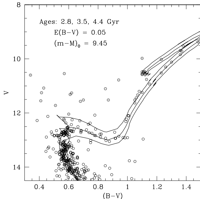
FIG. 5.—Comparison between the CMD of M67 (data from MMJ) and the isochrones from Girardi et al. (2000). The isochrones were transformed to the observational plane using the recipe described by Schiavon et al. (2002a) and the reddening and distance modulus indicated in the top left. From left to right: the ages of the theoretical isochrones are 2.8, 3.5, and 4.4 Gyr. The age that best fits the cluster data is 3.5 Gyr.
