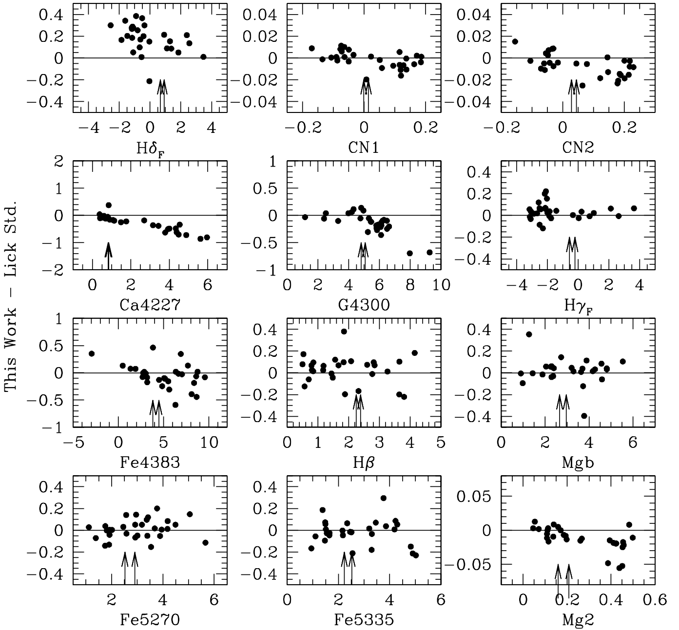
FIG. 2.—Comparison of the line indices measured in our spectra for Lick/IDS standards with the standard values. For all indices (except Ca4227) only minor zero-point corrections are needed to convert our data to the Lick/IDS system. The arrows indicate the values measured in the integrated spectra of M67 and M32, the main targets of this study, showing that they are in a locus in the index space that is very well populated by standard-star measurements. The error bars of our index measurements are about the same size as the symbols.
