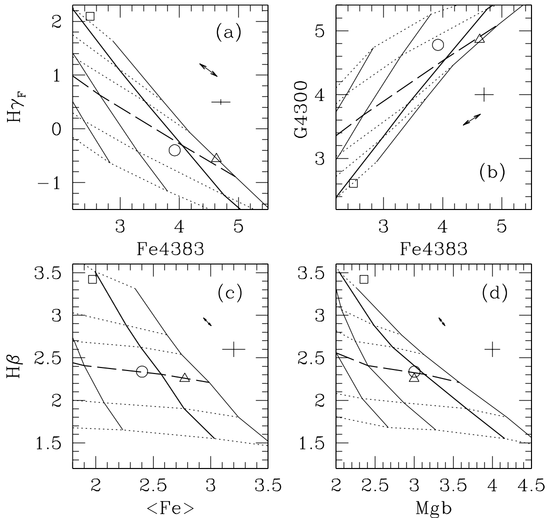
FIG. 7.—Same as Fig. 6. Symbols are the same as for Fig. 6. The most important conclusions to be drawn from this figure and Fig. 6 are (1) all Balmer lines indicate the same age for M67, in agreement with the CMD-based age; (2) the Fe, CN, and Mg indices indicate solar abundances within \pm 0.1 dex, in agreement with spectroscopic studies of stellar members; (3) when BSs are included in the integrated spectrum of M67, the spectroscopic age drops to \sim 1.2 Gyr, or even younger, depending on the line index adopted. For the G band the dependence on age is inverted, so that age decreases from top (14.1 Gyr) to bottom (2.0 Gyr). Ages based on the G band are too old (a factor of 2 in the case of M67). For M32, bluer Balmer lines tend to indicate younger ages, and bluer Fe lines indicate higher metallicities. The data on M32 indicate that it has supersolar iron abundance and is underabundant in magnesium relative to iron. See discussion in the text.
