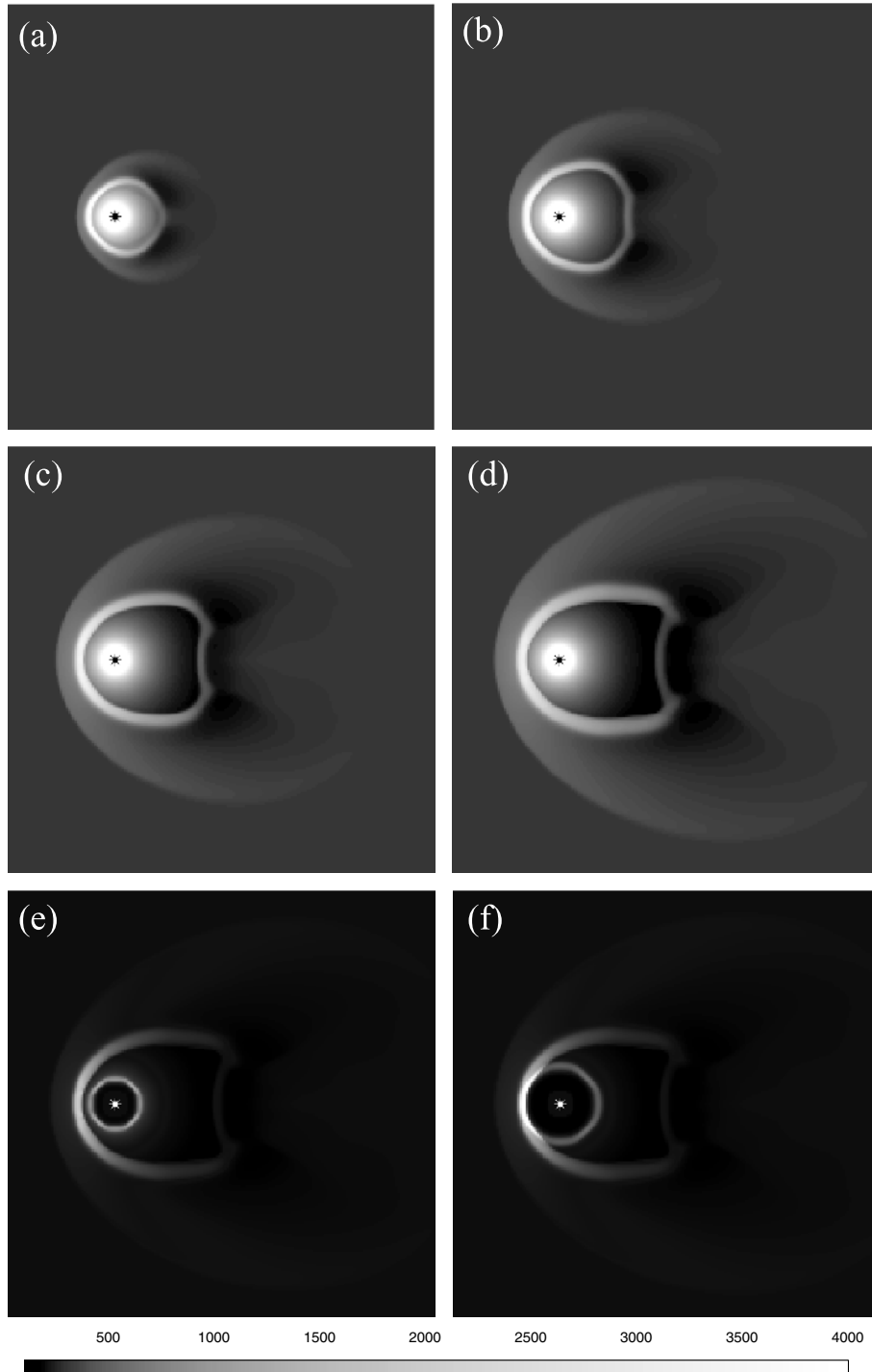
Figure 1. The results of case A: the panels show the gas density during the AGB and post-AGB phases. In panel (a), the simulation is 125 000 yr into the AGB phase, panel (b) 250 000 yr, panel (c) 375 000 yr, panel (d) 500 000 yr, panel (e) 15 000 yr into the post-AGB phase and in panel (f) 30 000 yr. The position of the central star is marked by an asterisk. The colour scaling is logarithmic and the density is scaled in units of 10^{-6} M_{\odot} \text{pc}^{-3} where 25 000 is equivalent to n_{\text{H}} = 1.0 \text{cm}^{-3} .
