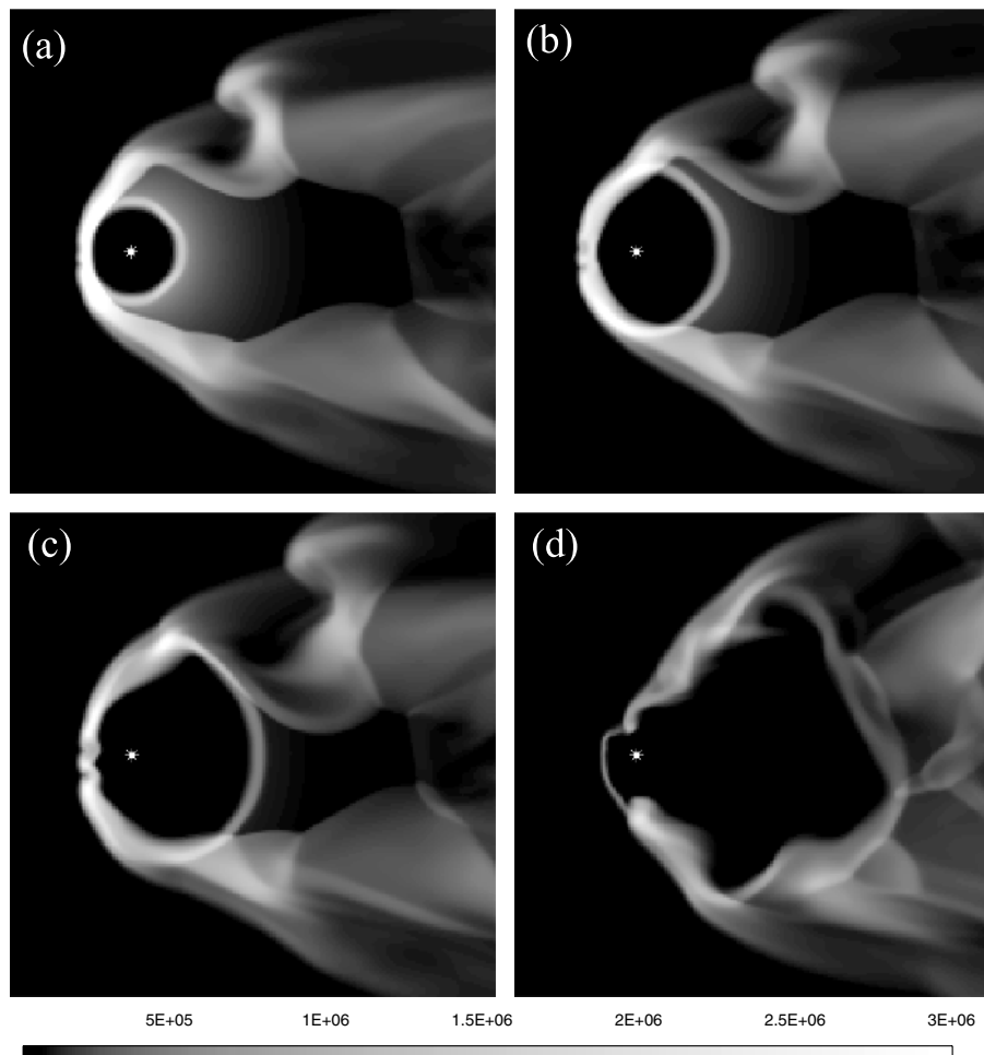
Figure 4. The results of case C: the panels show the gas density during the post-AGB phase. In panel (a), the simulation is 5000 yr into this phase, in panel (b) 10 000 yr, in panel (c) 15 000 yr and in panel (d) 30 000 yr. The position of the central star is marked by an asterisk. The colour scaling is logarithmic and the density is scaled in units of 10^{-6} M_{\odot} \text{pc}^{-3} , where 2.5 \times 10^6 is equivalent to n_{\text{H}} = 100 \text{ cm}^{-3} .
