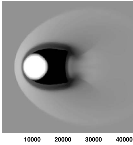
Figure 2. In this figure, we show the temperature profile (in K) of the 30 000-yr-old PN shown in panel (f) of Fig. 1 on the same slice through the numerical domain.
