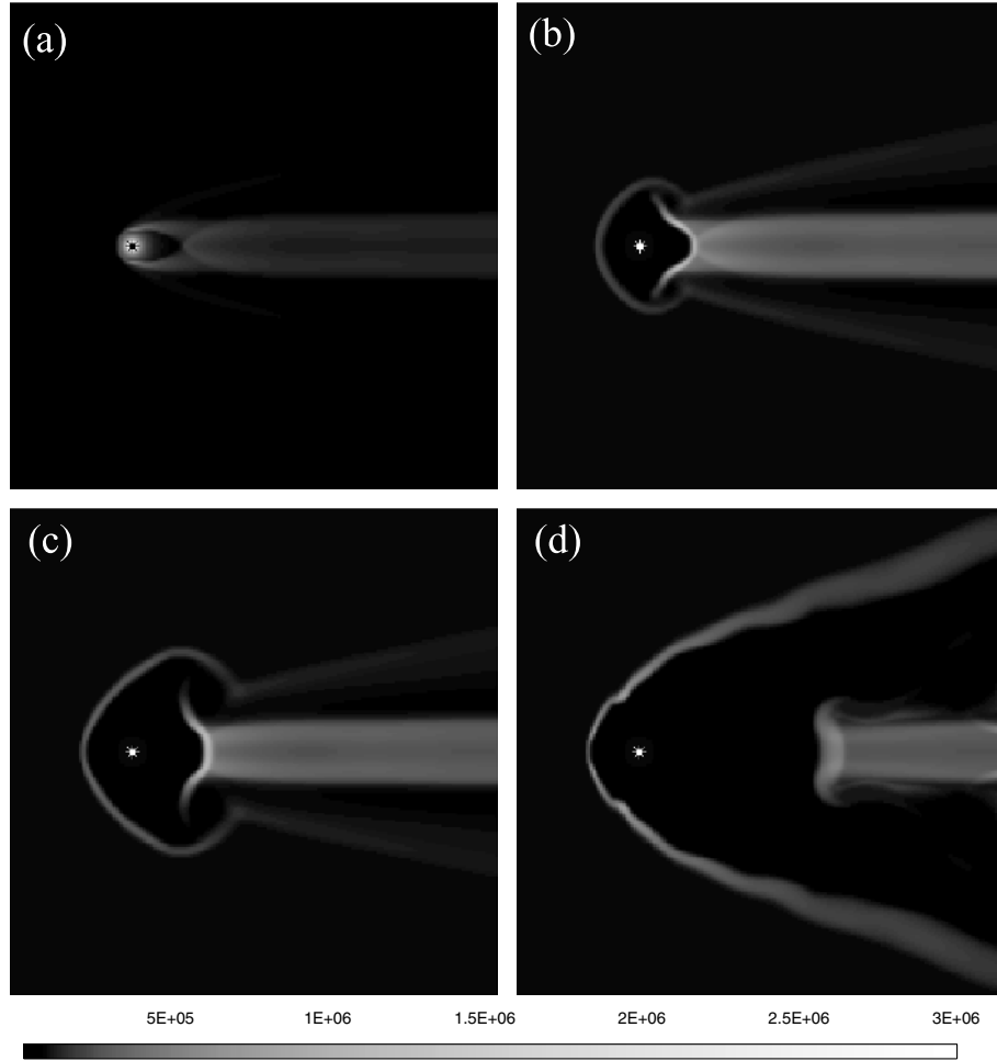
Figure 5. The results of case D: the panels show the gas density during the post-AGB phase. In panel (a), the simulation at the end of the AGB phase, in panel (b) 1000 yr into the post-AGB phase, in panel (c) 2000 yr and in panel (d) 10 000 yr. The position of the central star is marked by an asterisk. The colour scaling is logarithmic and the density is scaled in units of 10^{-6} M_{\odot} \text{pc}^{-3} , where 2.5 \times 10^6 is equivalent to n_{\text{H}} = 100 \text{cm}^{-3} .
