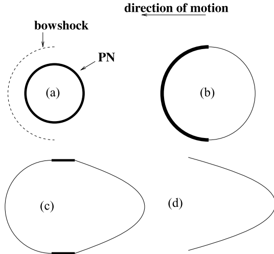
Figure 7. A simple illustration of the appearance of a PN during the four stages of PN–ISM interaction discussed in Section 5.1. The direction of motion is towards the left-hand side and the thicker lines indicate the brightest regions. Panel (a) illustrates stage WZO 1, (b) stage WZO 2, (c) stage WZO 3 and (d) stage WZO 4. The position of the letters (a), (b), (c) and (d) indicate the position of the central star at each stage.
