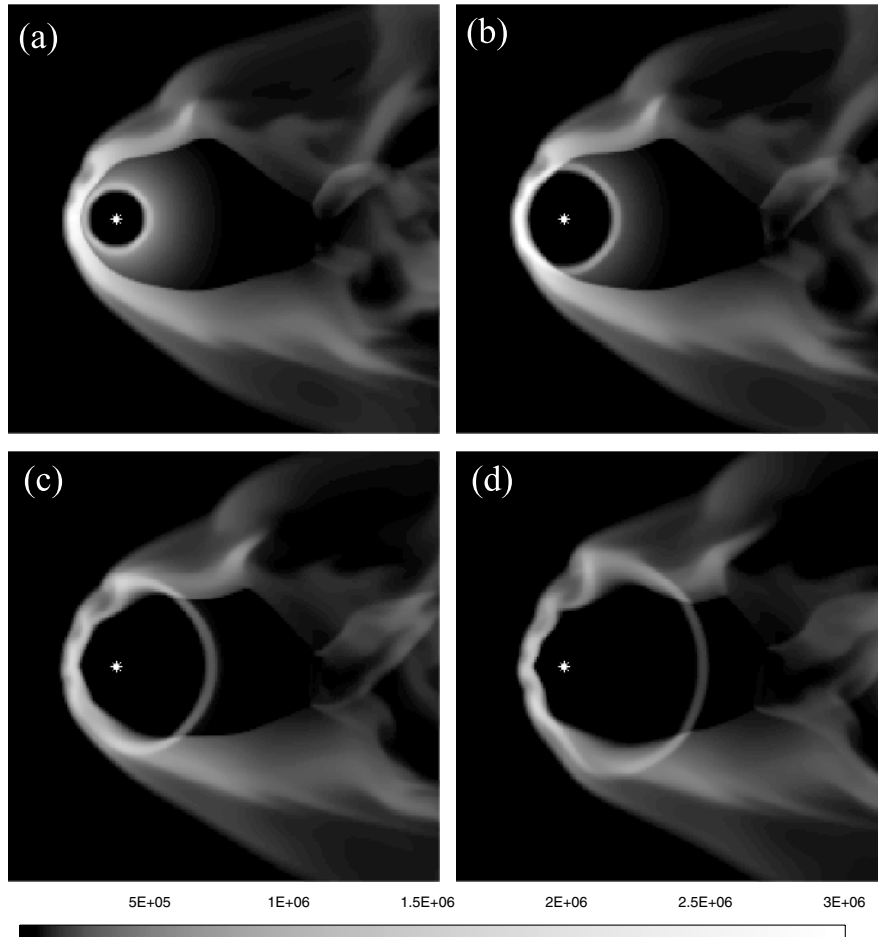
Figure 3. The results of case B: the panels show the gas density during the post-AGB phase. In panel (a), the simulation is 5000 yr into this phase, in panel (b) 10 000 yr, in panel (c) 20 000 yr and in panel (d) 30 000 yr. The position of the central star is marked by an asterisk. The colour scaling is logarithmic and the density is scaled in units of 10^{-6} M_{\odot} \text{pc}^{-3} , where 2.5 \times 10^6 is equivalent to n_{\text{H}} = 100 \text{cm}^{-3} .
