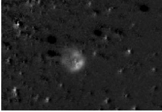
Figure 8. VLT FORS1 image in [O III] of the PN in NGC 6441. Continuum has been subtracted. The edge brightening is indicative of a PN–ISM shock.
