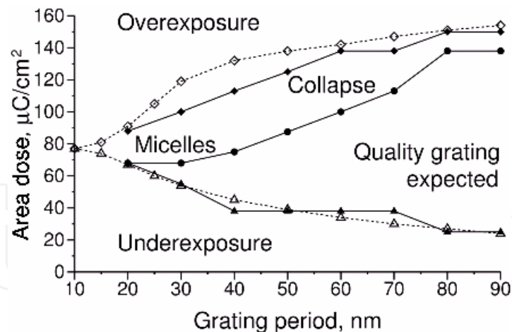
Fig. 4. Diagram of the characteristic morphologies in PMMA for various grating periods and area exposure doses using 10 keV voltage. Filled symbols show experimental results for the conditions as in Fig.1: triangles denote the boundary for underexposure (insufficient clearance); diamonds denote the boundary for overexposure (excessive clearance), and circles indicate the boundary for collapse or micellization. Open symbols show the results of numerical modeling of clearance as discussed in Sect. 3.2. (Mohammad et al., 2007).
