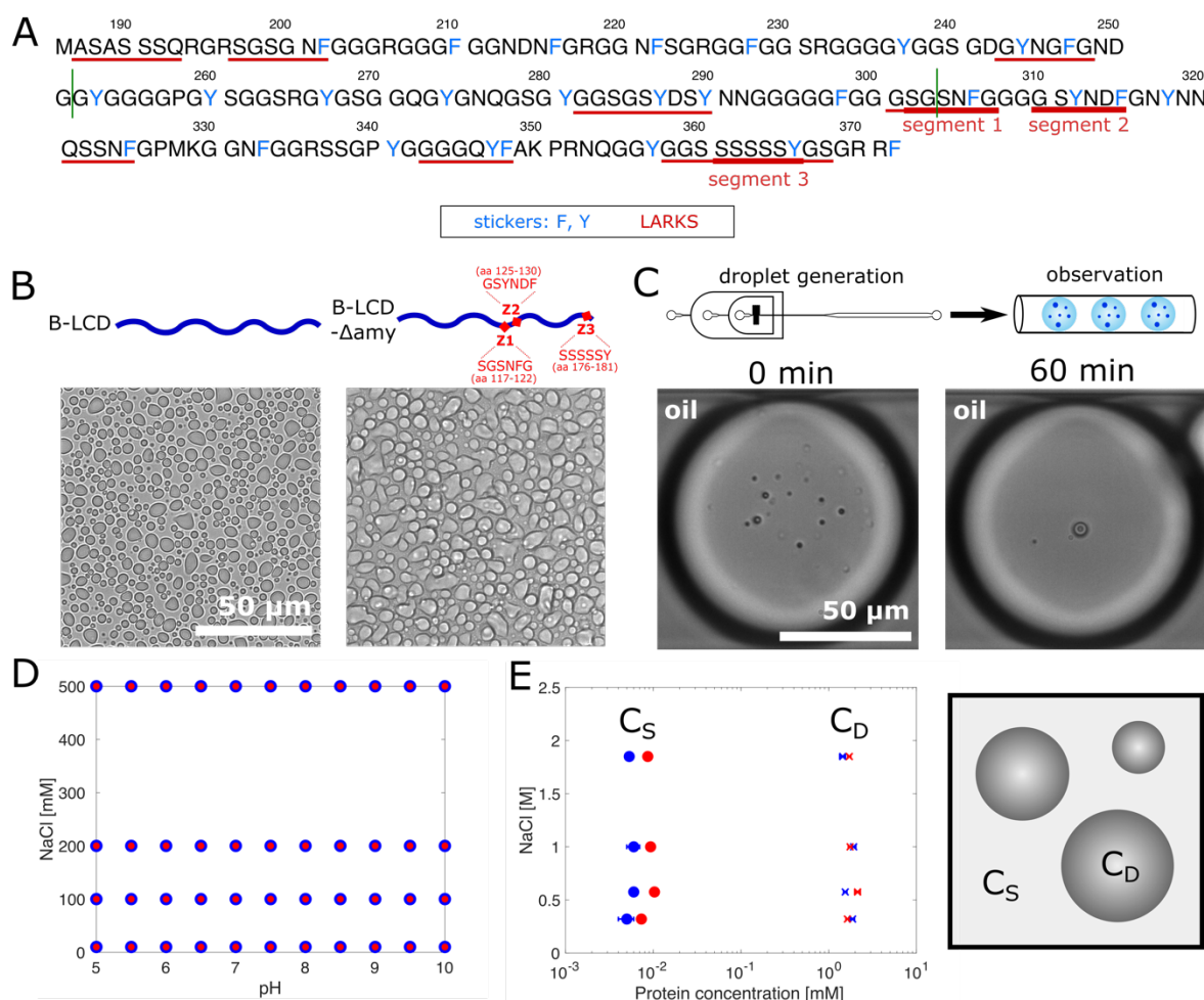
Figure 1: Liquid-liquid phase separation of B-LCD and zipper-depleted variant B-LCD- \Delta amy. (A) Sequence of the low-complexity domain of hnRNPA1-B (B-LCD). LCD of hnRNPA1-A (A-LCD) comprises amino acids 186-250 and 303-372 (borders indicated by green lines). Stickers (aromatic amino acids) are indicated in blue while fibril forming segments (steric zippers / LARKS) are underlined in red. (B) Brightfield microscopy images of droplets formed by B-LCD and zipper-depleted construct B-LCD- \Delta amy lacking three fibril forming segments ( \Delta SGSNFG, \Delta GSYNDF, \Delta SSSSY). (C) B-LCD droplets are liquid-like and merge in microfluidic water-in-oil droplet compartments until one single condensate is formed within 60 min. (D) Both B-LCD (blue circles) and B-LCD- \Delta amy (red circles) undergo LLPS under a broad range of ionic strength and pH values. Circles indicate presence of LLPS. (E) Protein concentrations inside ( C_D ) and outside ( C_S ) the droplets at different ionic strengths are similar for B-LCD (blue) and B-LCD- \Delta amy (red). Error bars represent the standard deviation of the average protein concentration inside and outside the droplets, obtained by measuring 3 different droplets (for C_D ) and 3 independent (for C_S ) samples at each NaCl concentration. When not visible, the error bars are smaller than the symbol.
