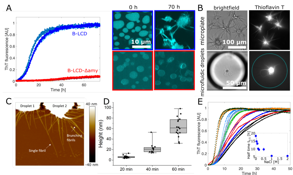
Figure 2: Liquid-amyloid transition of hnRNPA1-B is governed by fibril forming segments (A) Fluorescence Thioflavin T (ThT) signal over time for B-LCD (blue) and B-LCD- \Delta Amy (red). Re-scan confocal microscopy images at time zero and after 70 hours of incubation for the two constructs. Each curve represents the normalized ThT fluorescence of one independent sample. (B) ThT-stainable star-shaped aggregates formed by B-LCD in microplates and in microfluidic water-in-oil droplets imaged in brightfield and by widefield fluorescence microscopy after 6 days of incubation. (C) Atomic Force Microscopy (AFM) of star-shaped aggregates formed by B-LCD after 1 h. (D) Increase of fibril height over 60 min after formation, extracted from AFM images. (E) Acceleration of amyloid formation in 30 \mu M B-LCD sample with increasing NaCl concentration. Inset: half time t_{0.5} values as a function of NaCl concentration (0 mM NaCl – black, 50 mM NaCl – blue, 100 mM NaCl – red, 150 mM NaCl – light green, 200 mM NaCl – grey, 500 mM NaCl – light blue, 1 M NaCl – orange, 2 M NaCl – dark green).
