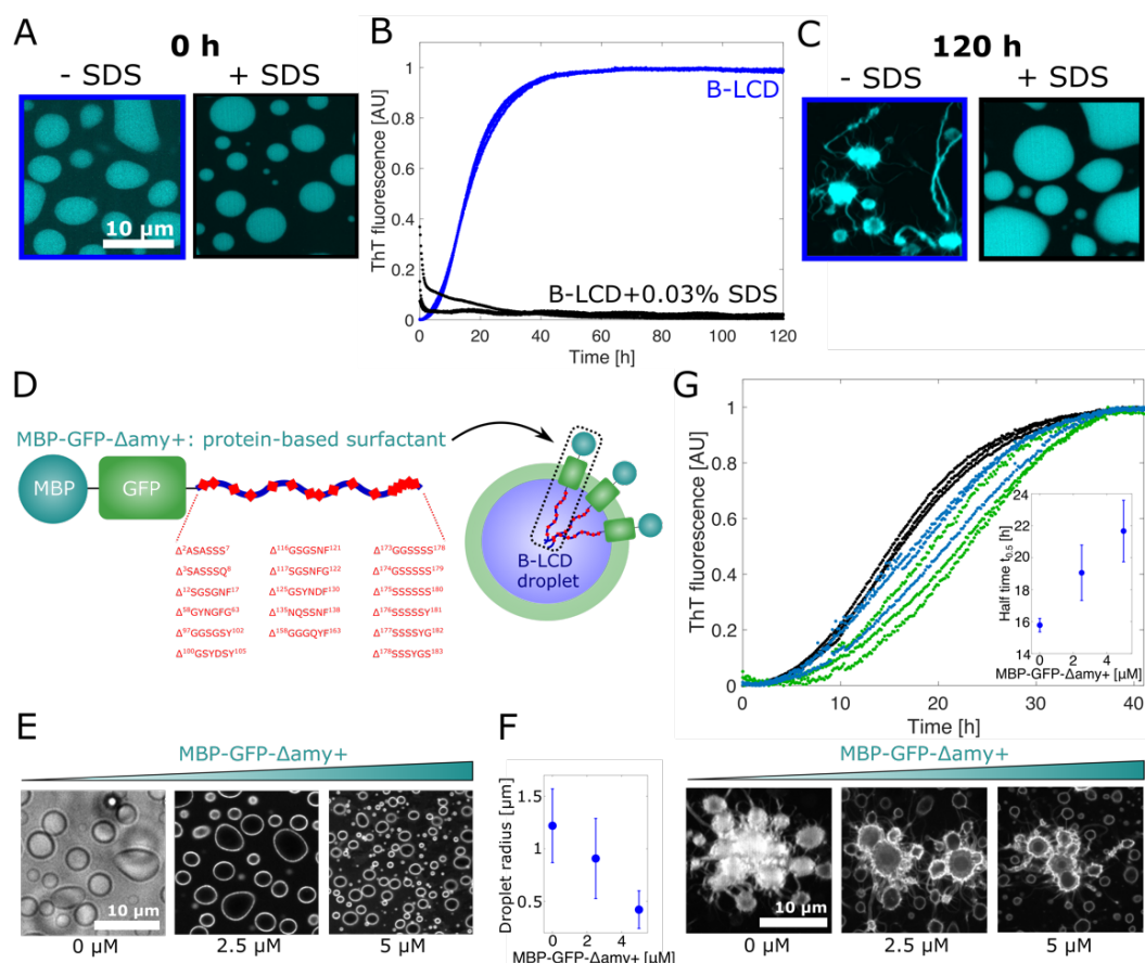
Figure 5: Targeting the surface of condensates inhibits amyloid formation. (A-C) The addition of 0.03% SDS to a 30 \mu\text{M} B-LCD solution did not affect LLPS (A) but prevented the increase of ThT signal over time (B) as well as the formation of rims and star-shaped aggregates after 120 h, as shown by re-scan confocal microscopy images (C). (D) Design of a protein-based surfactant (MBP-GFP- \Delta\text{amy}^+ ) consisting of soluble Maltose-binding protein (MBP), Green-fluorescent protein (GFP) and a B-LCD variant lacking all predicted steric zippers ( \Delta\text{amy}^+ ). (E) Re-scan confocal fluorescence microscopy images showing accumulation of the protein-based surfactant molecules at the droplet surface. The fluorescent signal is originating from the GFP domain of the protein surfactant. Images were acquired at time 0. (F) Decrease of the average droplet size with increasing MBP-GFP- \Delta\text{amy}^+ concentration. Error bars represent the standard deviation of sizes of > 1000 droplets from 3 independent samples. (G) In addition to changing the size of the condensates, increasing concentrations of the protein-based surfactant delays amyloid formation inside condensates. The inset depicts the average half times t_{0.5} extracted from the ThT profiles as a function of the MBP-GFP- \Delta\text{amy}^+ protein surfactant. Black – 0 \mu\text{M} MBP-GFP- \Delta\text{amy}^+ , blue – 2.5 \mu\text{M} MBP-GFP- \Delta\text{amy}^+ , green – 5 \mu\text{M} MBP-GFP- \Delta\text{amy}^+ . Error bars represent the standard deviation of three independent samples. Re-scan confocal fluorescence microscopy images of samples after 40 h of incubation with increasing protein surfactant concentration.
