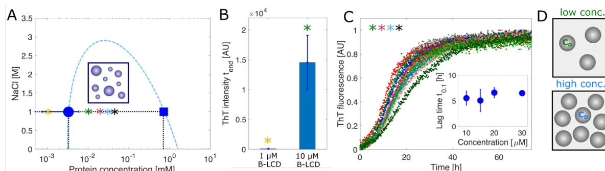
Figure 3: Condensation of hnRNPA1-B LCD accelerates amyloid formation. (A) Protein concentration inside ( C_D , blue square) and outside ( C_S , blue circle) the droplets. Asterisks indicate initial protein concentration in kinetic experiments in (B) and (C): 1 \mu M (yellow), 10 \mu M (green), 15 \mu M (red), 20 \mu M (blue), 30 \mu M (black). Error bars represent the standard deviation of the average protein concentration inside and outside the droplets, obtained by measuring 3 different droplets (for C_D ) and 3 independent samples (for C_S ) at each C_0 . The blue dashed line represents a guide to the eyes. (B) ThT fluorescence intensity value of 1 \mu M and 10 \mu M B-LCD solutions after 7 days incubation, respectively below and above the critical concentration of LLPS ( C_c = 2.5 \mu M). (C) Normalized ThT kinetic profiles corresponding to the initial protein concentrations C_0 in (A). The inset shows the average lag times t_{0.1} at various initial protein concentrations C_0 . Error bars represent standard deviation of three independent samples. (D) Droplets formed at low and high initial B-LCD concentration exhibit similar internal protein concentration ( C_D ) but increase in number when the initial protein concentration is increased.
