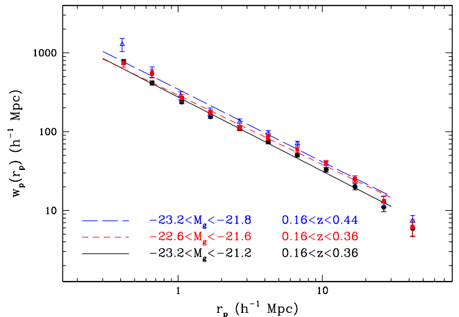
FIG. 10.— Projected correlation function w_p(r_p) for the three LRG samples discussed in the paper, plotted together with power-law fits fitted over the range 0.3 < r_p < 30h^{-1} \text{ Mpc} .
