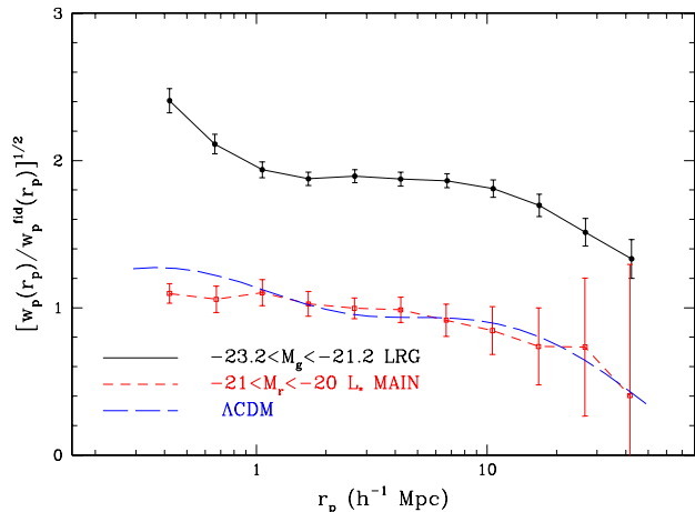
FIG. 9.— [w_p(r_p)/w_p^{fid}(r_p)]^{1/2} as a function of separation r_p for the -23.2 < M_g < -21.2 LRG sample (solid symbols and line) and for the L_* MAIN galaxy sample (open symbols and short-dashed line; Zehavi et al. 2004b), allowing to infer their relative bias. w_p^{fid}(r_p) is the projected correlation function corresponding to a fiducial power-law \xi(r) = (r/5h^{-1} \text{ Mpc})^{-1.8} . The long-dashed curve shows this relative quantity for a \Lambda CDM cosmology computed from the nonlinear power spectrum of Smith et al. (2003).
