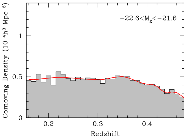
FIG. 3.— As Figure 1, but for the -22.6 < M_g < -21.6 sample. The sample is close to a constant comoving volume for z < 0.36 .
