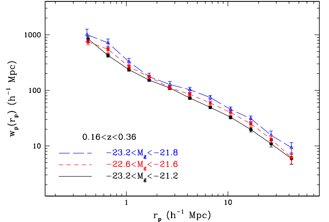
FIG. 13.— Luminosity dependence of w_p(r_p) obtained for the three LRG samples for 0.16 < z < 0.36 .
