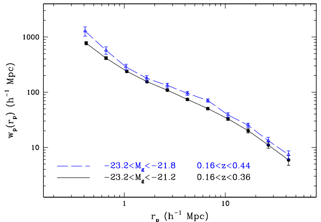
FIG. 6.— Projected correlation function w_p(r_p) for the LRG samples.
