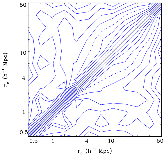
FIG. 7.—Normalized error covariance matrix for the w_p(r_p) measurement of the -23.2 < M_g < -21.2 sample. The normalized covariance matrix is defined as C_{ij}/(C_{ii} \cdot C_{jj})^{1/2} , where C_{ij} are the elements of the error covariance matrix. Contour spacing is 0.1 going from 1 on the diagonal (thick line) down to 0. The dashed lined denotes the 0.5 contour. Tickmarks denote the elements in the covariance matrix, and the labels denote the corresponding r_p values.
