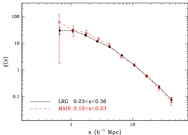
FIG. 5.— Redshift-space correlation function \xi(s) for the -22.6 < M_g < -21.6 passively-evolved LRG sample and the comparable one from the MAIN galaxy sample.
