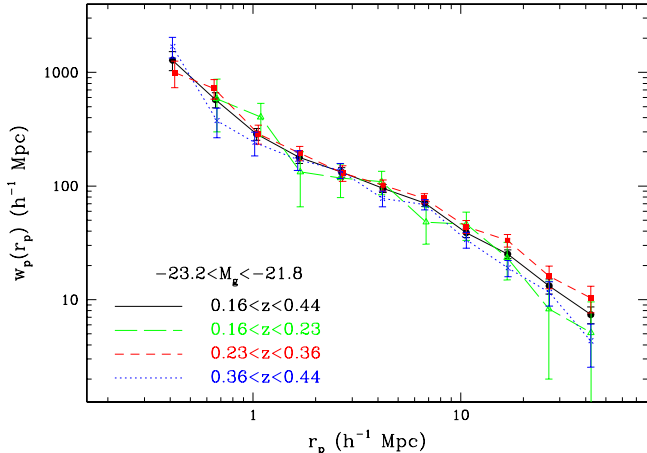
FIG. 12.— Redshift dependence of the w_p(r_p) clustering results for the -23.2 < M_g < -21.8 sample.
