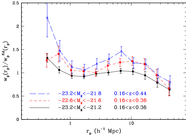
FIG. 11.— Projected correlation function w_p(r_p) for the LRG samples shown in Fig. 10, now all divided out by a fiducial power-law w_p(r_p) corresponding to \xi(r) = (r/10h^{-1} \text{ Mpc})^{-1.9} . The deviations from a power-law are clearly visible.
