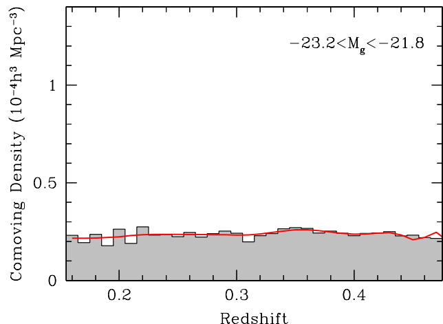
FIG. 2.— As Figure 1, but for the -23.2 < M_g < -21.8 sample. The sample is close to a constant comoving volume for z < 0.44 .
