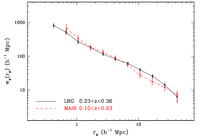
FIG. 8.—Projected correlation function w_p(r_p) for the -22.6 < M_g < -21.6 LRG sample and the comparable one from the MAIN galaxy sample.
