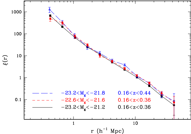
FIG. 14.— Real-space correlation function \xi(r) for the three LRG samples.
