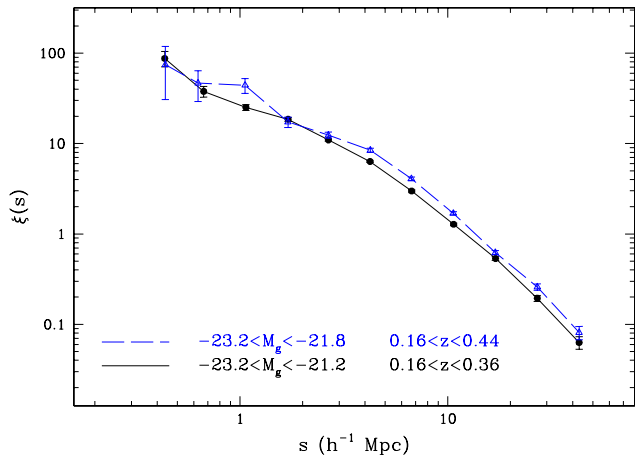
FIG. 4.— Redshift-space correlation function \xi(s) for the LRG samples. Bins in s are in logarithmic separation of 0.2.
