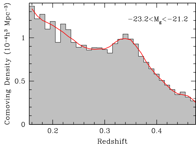
FIG. 1.— The comoving number density of the -23.2 < M_g < -21.2 sample. The shaded histogram is the distribution of the actual data, and the solid continuous line is our model for the redshift distribution, described in Appendix A. The sample is close to a constant comoving volume for z < 0.36 , although the fluctuations are reaching about 30% peak-to-peak (but one should note that the lowest redshifts, where the excess is, contain less volume than the redshift range would suggest).
