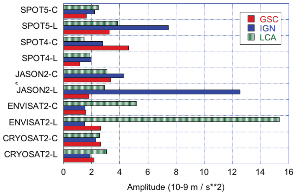
Figure 4 RMS of DORIS empirical parameters (once-per-revolution) estimated by satellite (in 2012), cross-track (C), and along-track (L).
