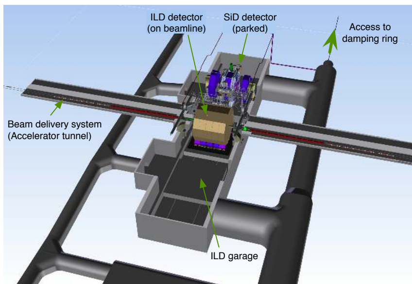
Figure 4.1 Example layout of the detector hall for the Mountain Topography site, showing the location of the two detectors in a push-pull arrangement.
