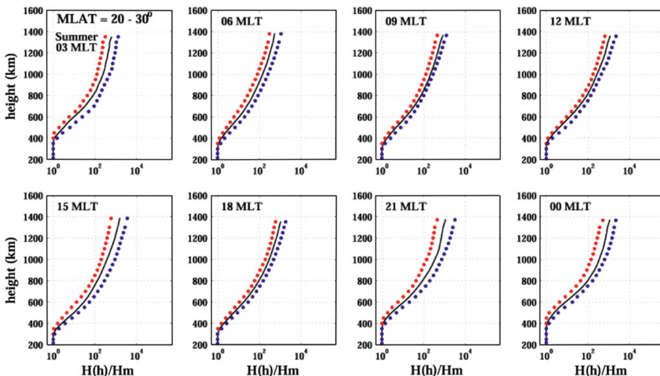
Fig. 4 Median H_n functions (black line) for magnetic latitudes between 20^\circ and 30^\circ for summer at different magnetic local times (MLT). The red and blue dots are the lower and upper quartiles
