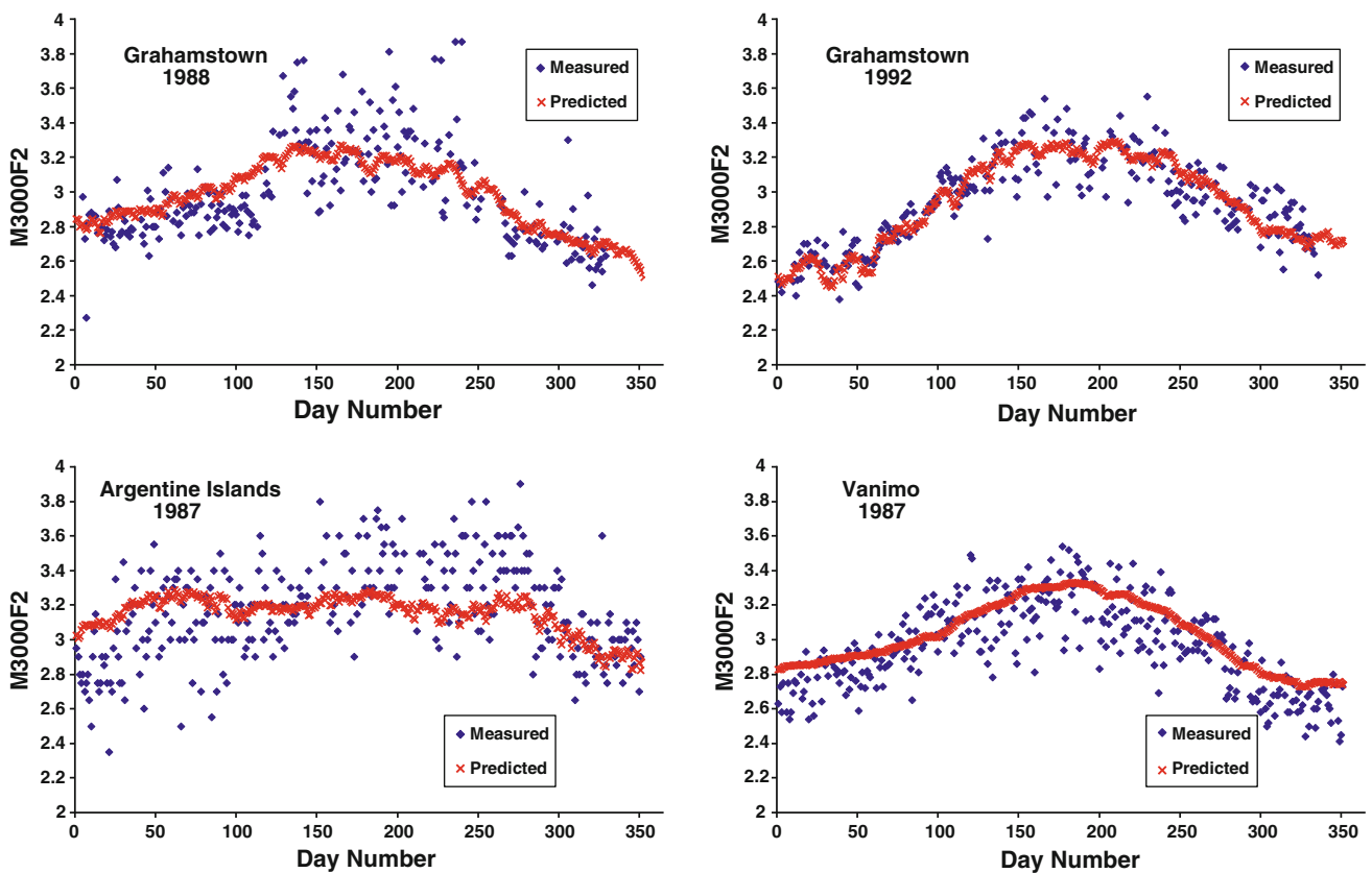
Fig. 2 Measured and predicted M(3000)F2 values for four example stations and years representing three latitude zones at 10h00 UT
