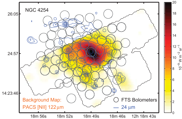
Figure 1. PACS [N II] 122 \mu\text{m} image of NGC 4254. The color scale shows the surface brightness in units of 10^{-9} \text{ W m}^{-2} \text{ sr}^{-1} . The black contours delineate the areas where [N II] 122 \mu\text{m} was observed, and the blue contours show the 24 \mu\text{m} dust continuum emission. The gray circles show the distribution of the 17" SPIRE-FTS bolometers used to detect the [N II] 205 \mu\text{m} line. The axes show the R.A. (J2000) and decl. (J2000) position coordinates.
