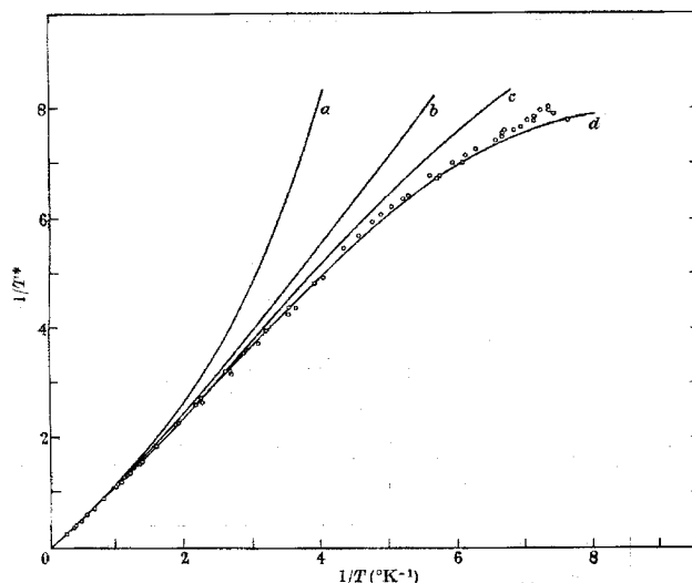
Figure 1. Variation of 1/T^* (= \chi/\lambda) against 1/T for dysprosium ethyl sulfate. The points (o) represent experimental results. The curves represent the results of various theoretical models. (a) Molecular field model; (b) Van Vleck expansion to second order (Eq. 2); (c) Ising model with nearest neighbor interactions in a molecular field due to other neighbors; (d) Ising model with nearest and next nearest neighbor interaction in a molecular field. After Ref. 11.
