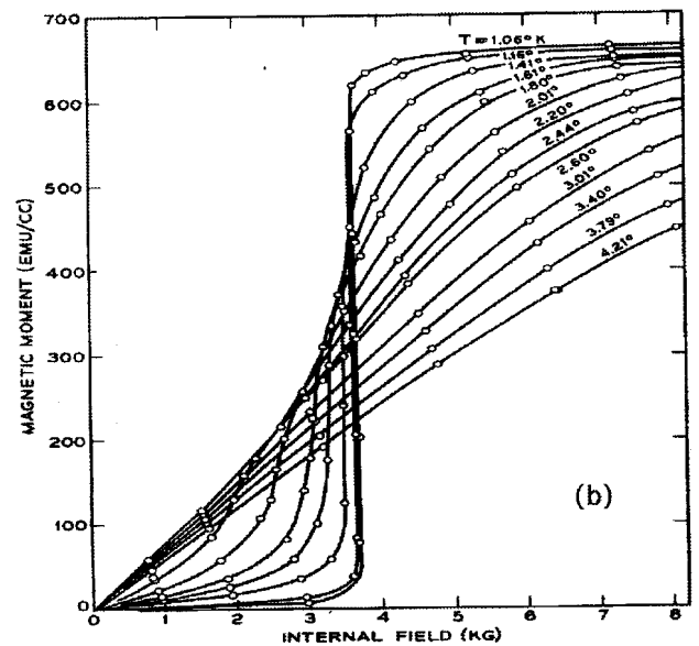
Figure 14. The magnetization of a spherical sample of DyAG as a function of field along [111] at temperatures above and below the Néel temperature. In (a) the magnetization is plotted as a function of the externally applied field. In (b) the magnetization is plotted as a function of the internal field, calculated by H_{int} = H_{ext} - NM , with N = 4\pi/3 for a sphere. After Ref. 49.
