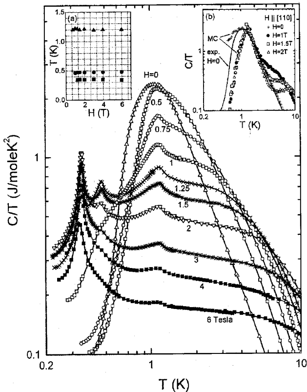
Figure 19. Specific heat as a function of temperature for Dy_2Ti_2O_7 in various applied fields. The broad H = 0 feature is suppressed on increasing H and replaced by three sharp features at 0.34, 0.47 and 1.12K. Inset (a) shows the constancy of these transition temperatures with field. Inset (b) shows the result of finite-field Monte Carlo simulations of C/T . After Ref. 71.
