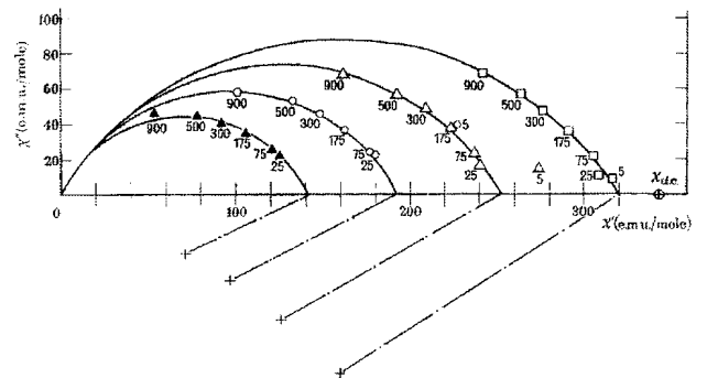
Figure 20. A plot of the out-of-phase susceptibility \chi'' as a function of the in-phase \chi' for DyES for various frequencies at four different temperatures. The frequency of measurement, in Hz, is written beside each symbol. The curves are circles which pass through the origin and best fit the data. The extrapolated values of \chi' for \chi'' = 0 are clearly different from the measured d.c. value, \chi_{d.c.} . After Ref. 75.
