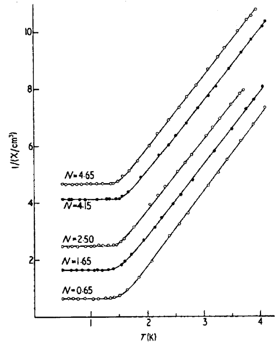
Figure 11. The reciprocal susceptibility parallel to the crystal c-axis as a function of temperature for \text{LiHoF}_4 . The experimental points correspond to measurements for five different sample shapes, characterized by demagnetizing factors, N . The constant values for T < 1.5\text{K} correspond to a transition to the ferromagnetic state, for which 1/\chi_{N=0} = 0 . After Ref.31.
