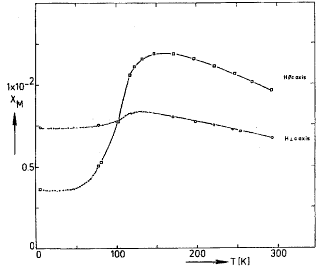
Figure 8. Magnetic susceptibility as a function of temperature for K_2CoF_4 , without any corrections. Note the differences from Fig. 6 and the large susceptibility perpendicular to the axis reflecting the influence of low-lying states and corresponding deviations from the simple Ising Hamiltonian. After Ref. 21.
