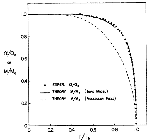
Figure 5. Spontaneous sublattice magnetization as a function of temperature for DyPO 4 . The points (o) represent experimental results of magneto-electric measurements; the two solid lines represent the results of a calculation based on a low- temperature series expansion with one adjustable constant, and a fit to a power-law with a fitted critical exponent \beta = 0.314 . The broken line represents the molecular field theory. After Ref. 16.
