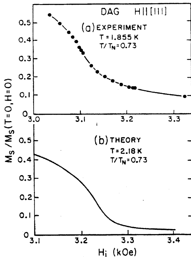
Figure 15. Results for the staggered magnetization, M_s , for DyAlG as a function of the internal field with H_i \parallel [111] . (a) Experimental results of Blume et al. [Ref. 53]; (b) results of the cluster calculation for the same value of T/T_N . After Ref. 55.
