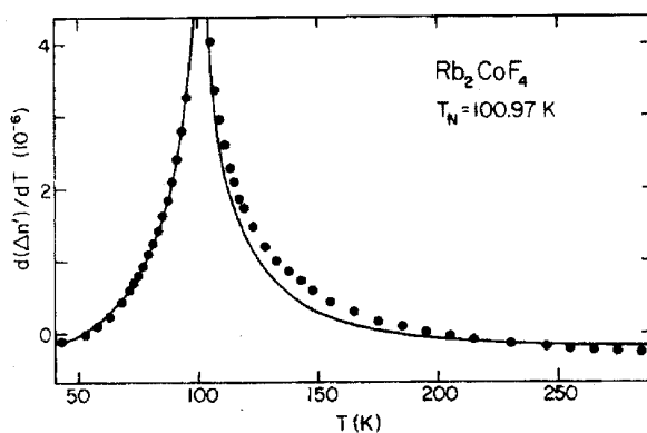
Figure 7. Variation of the magnetic specific heat, as a function of temperature for Rb_2CoF_4 . The solid points (•) are experimental results of optical birefringence measurements shown previously to be proportional to the magnetic specific heat. The solid line is the exact Onsager solution for the two-dimensional Ising model with amplitude and critical temperature adjusted to fit the data, and a small constant background term subtracted. After Ref. 22.
