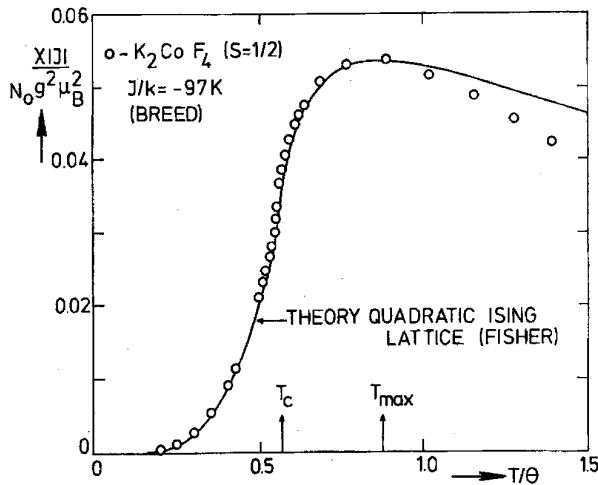
Figure 6. Magnetic susceptibility parallel to the axis as a function of temperature for K_2CoF_4 . The points (o) represent experimental results (Ret: 21) corrected for a temperature independent Van Vleck contribution to make \chi = 0 at T = 0K . The solid line represents the series expansion of Sykes and Fisher for the quadratic S = 1/2 Ising antiferromagnet fitted with one adjustable constant. After Ref. 6.
