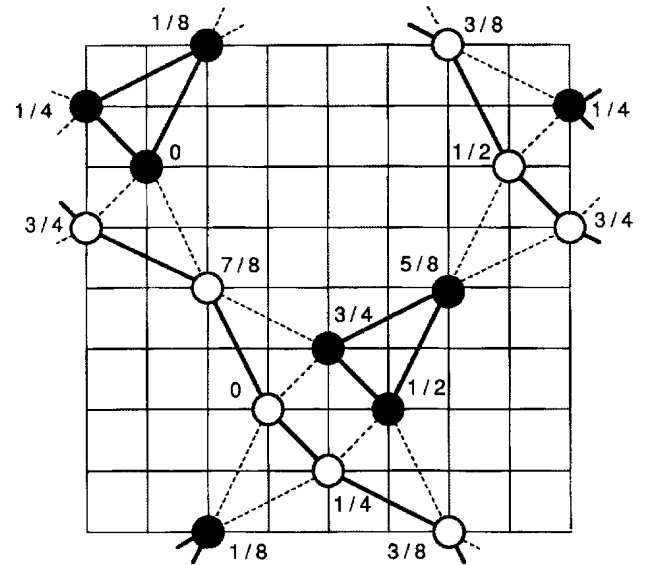
Figure 16. Lattice and bond structure of the staggered interaction model shown in a [001] projection. The structure is body centered cubic, with 6 sites in the primitive unit cell. The figure shows the conventional unit cell. The numbers give the heights above the z = 0 plane in terms of the unit-cell edge length. Ferromagnetic bonds are shown as solid lines and antiferromagnetic bonds are shown as broken lines. Note that only half the sites, marked as (\bullet) , form triangles with three ferromagnetic bonds, whereas the sites marked (o) have only two ferromagnetic bonds. The structure shown corresponds to one half of the sites in DyAlG. The omitted sites form a similar lattice related by simple translations and do not share any nearest neighbor bonds with the sites shown. After Ref. 55.
