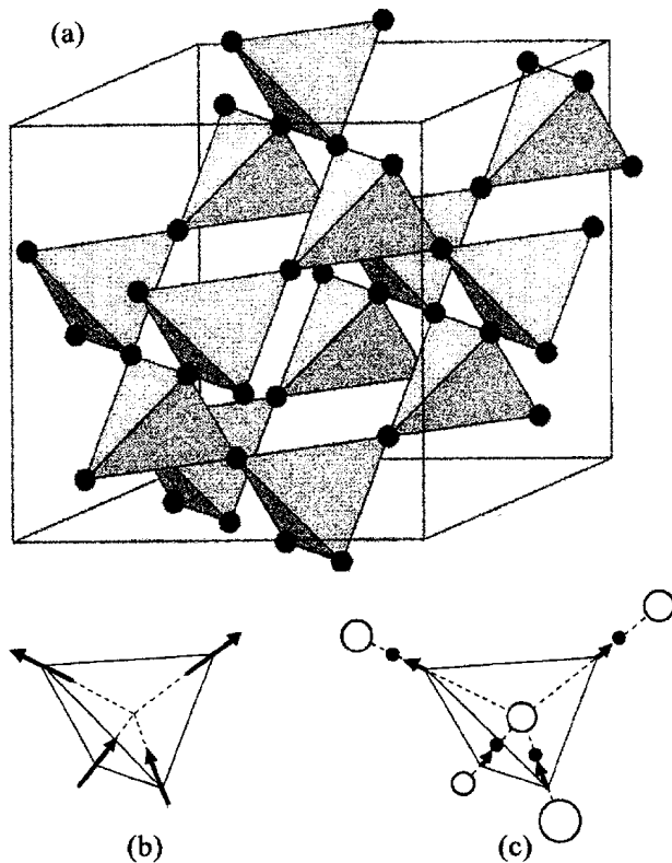
Figure 17. (a) A schematic representation of the pyrochlore lattice, showing the positions of the magnetic ions. (b) The ground state of a single tetrahedron of spins coupled ferromagnetically with local Ising anisotropy. (c) Local proton arrangement in ice, showing the oxygen atoms ( \bullet ) and hydrogen atoms ( - ), and with the displacement of the hydrogen atoms from the mid-points of the oxygen-oxygen bonds marked by arrows. The similarity to (b) has led to the concept of 'spin-ice.' After Refs. 67 and 73.
