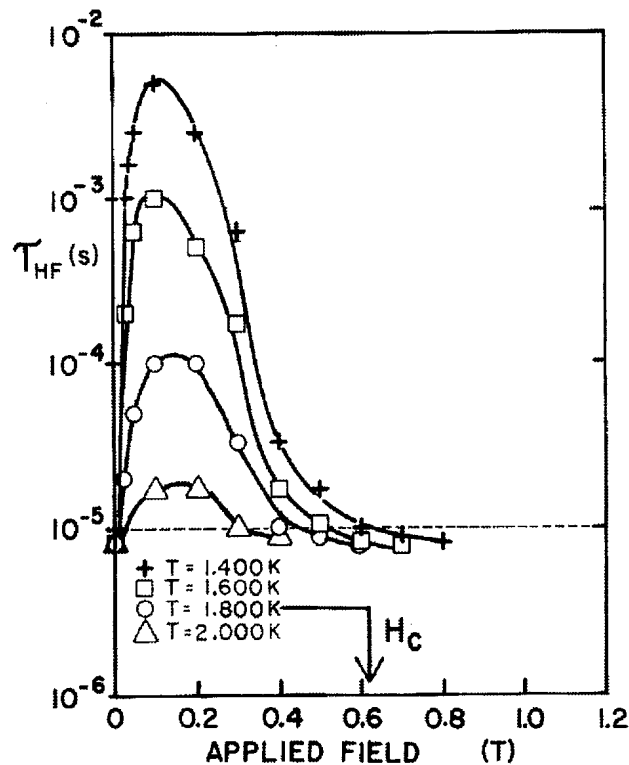
Figure 21. Field and temperature dependence of one of the relaxation times, IHF, of DyAlG. The arrow indicates the location of the phase boundary H_c at 1.8 K; at the other temperatures shown H_c is not very different. All the results therefore correspond to measurements in the antiferromagnetic phase. The broken line at 10^{-5} indicates the lower limit of the measurements. After Ref. 83.
