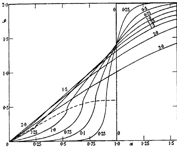
Figure 13. The magnetization as a function of magnetic field at fixed temperature for a two-dimensional super-exchange antiferromagnet. The dashed curve is the locus of transition points. The curves are labeled by appropriate values of the reduced temperature. Note the continuity of all curves except for zero temperature, and the infinite derivative at the transition points. After Ref. 48.
