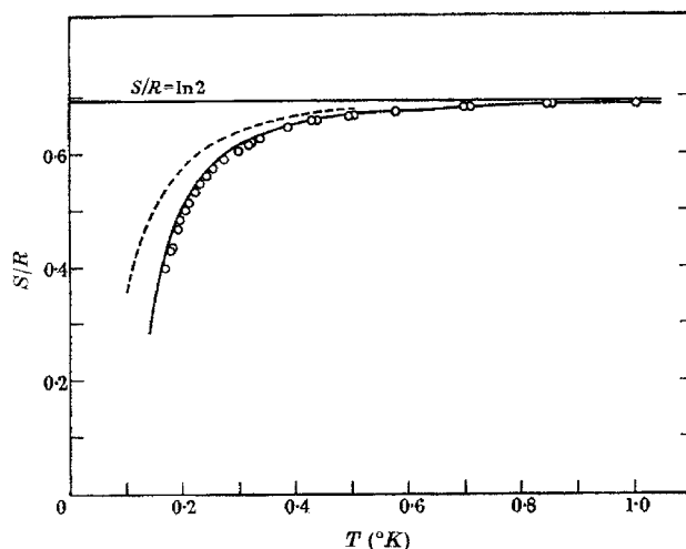
Figure 2. Entropy of dysprosium ethyl sulfate as a function of temperature. The points (o) represent experimental results. The broken line represents a model assuming non-interacting linear Ising chains and the solid lines the results predicted by the Oguchi cluster expansion method. After Ref. 11.
