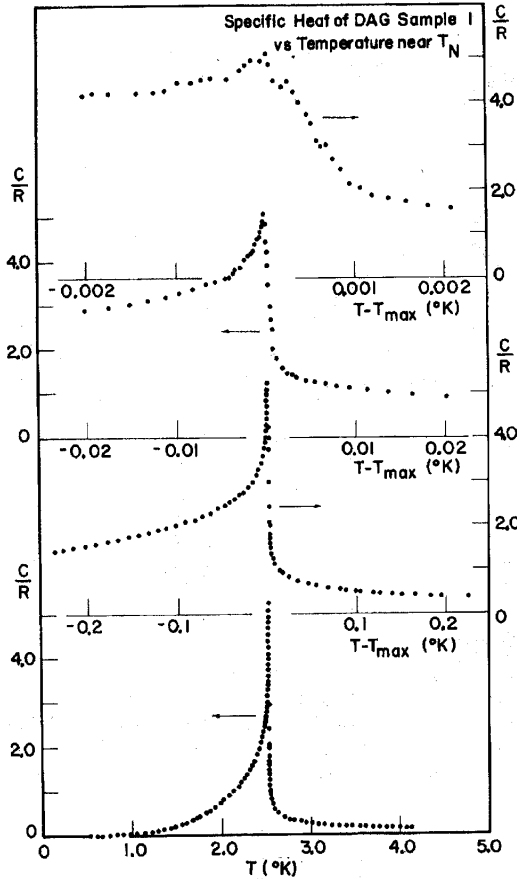
Figure 10. Specific heat of \text{Dy}_3\text{Al}_5\text{O}_{12} as a function of temperature near T_N , under four decades of temperature resolution. Temperatures are measured relative to an arbitrarily chosen T_{\text{max}} = 2.544 K. After Ref. 26.
