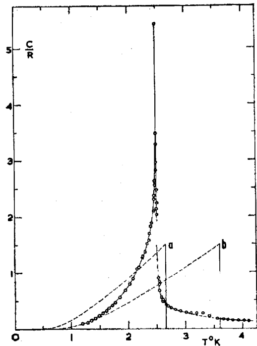
Figure 9. Specific heat as a function of temperature for Dy 3 Al 5 O 12 . The points (o) represent experimental results. Curves (a) and (b) were calculated using the mean field approximation, with the constant for (a) estimated on the basis of pure magnetic dipole-dipole interaction, and for (b) by fitting the low-temperature experimental points. After Ref. 24.
