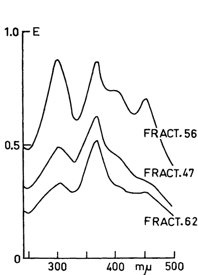
Fig. 5. Sulphuric acid spectra of active material (fractions from K 25) from the chromatography shown in Fig. 4. The fraction numbers refer to this figure.
