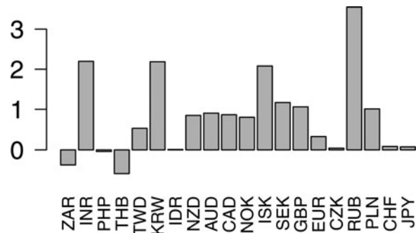
Figure 8. Multivariate stochastic volatility model: differences between post-crisis and pre-crisis posterior expectation of the parameter m for the 20 currencies.
