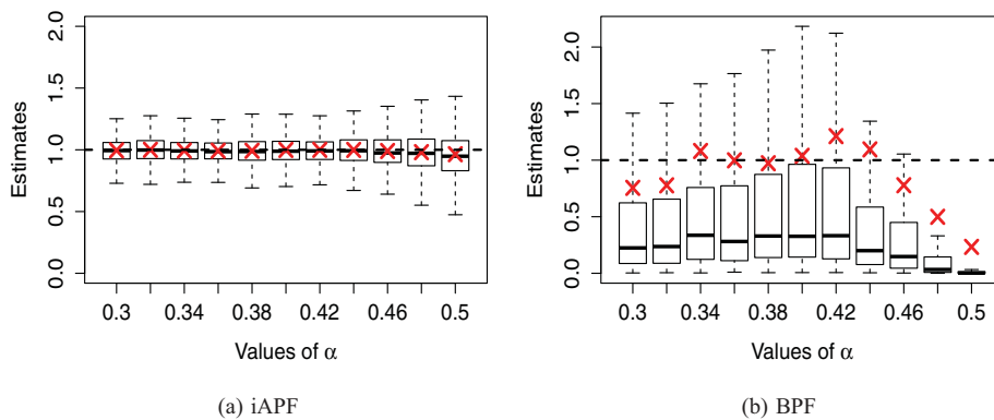
Figure 2. Boxplots of \hat{Z}/Z for different values of the parameter \alpha using 1000 replications. The crosses indicate the mean of each sample.
