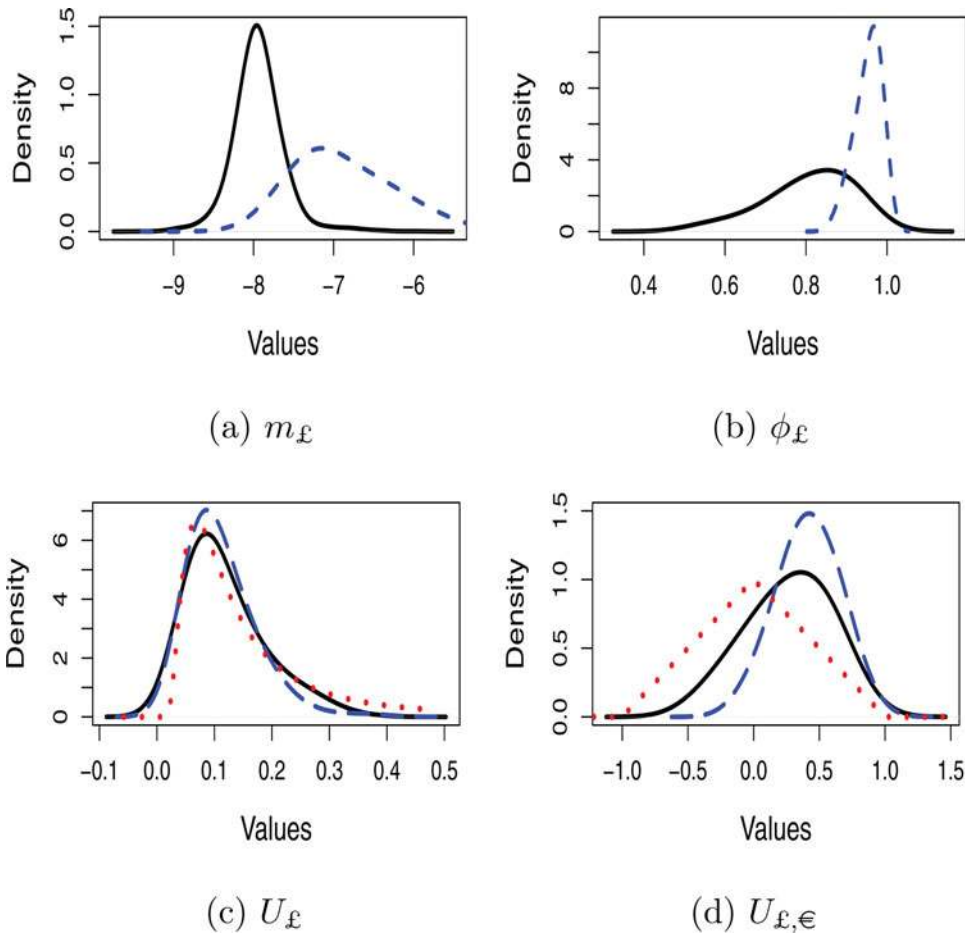
Figure 7. Multivariate stochastic volatility model: density estimates for the parameters related to the Pound Sterling. Pre-crisis chain (solid line), post-crisis chain (dashed line), and prior density (dotted line). The prior densities for (a) and (b) are constant.
