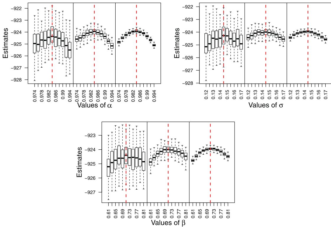
Figure 6. Log-likelihood estimates in a neighborhood of the MLE. Boxplots correspond to 100 estimates at each parameter value given by three particle filters, from left to right: BPF ( N = 1000 ), BPF ( N = 10,000 ), iAPF ( N_0 = 100 ).
