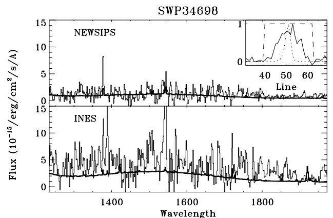
Fig. 5. Example of the differences in the extraction of a weak extended source. The use of a boxcar extraction in the whole aperture for weak sources guarantees that all the flux will go into the extracted spectrum. Symbols are as in 4
