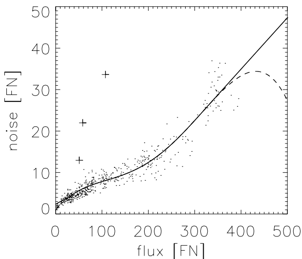
Fig. 1. Example of the noise model for the wavelength 1612 Å. Points represent the standard deviation \sigma(FN) as a function of the corresponding median flux numbers \langle FN \rangle_0 . The crosses indicate data not considered for the modeling. The continuous line shows the noise model applied in INES consisting of a fitted polynomial and its linear extrapolation. The broken line shows the SWET extrapolated polynomial for comparison
