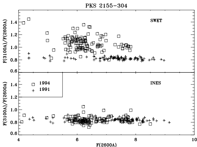
Fig. 14. The 3100 Å region in the SWET extracted spectra of PKS 2155–304 ( upper panel ) is strongly contaminated by solar scattered light as shown by the ratio F(3100 \text{ Å})/F(2600 \text{ Å}) in 1994 ( squares ) and 1991 ( crosses ). The values of this ratio during 1994 and 1991 are in much better agreement when INES extracted spectra are used ( lower panel )
