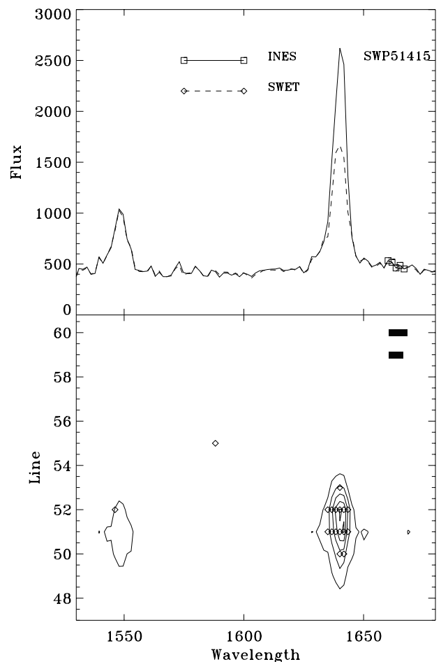
Fig. 7. Example of the extraction with INES and SWET of a spectrum with weak continuum and strong narrow emission lines in. The HeII 1640 Å line is not flagged in either of the extracted spectra. Shown in the bottom panel is the bi-dimensional SILO file with the 2-D quality flags overplotted. Diamonds correspond to flag “-32” ( SWET Cosmic ray) and filled squares to other flags (e.g. reseau marks)
