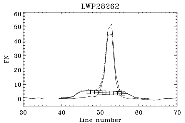
Fig. 11. The thick line shows the average spatial profile from 2900 Å to 3300 Å in the image LWP28262. The contribution from the solar scattered light contamination and the extraction profile used for the point source are shown as thin lines and the sum of both is represented by crosses. Squares show the extrapolated points of the solar contribution. Note that there is still some remnant contribution of the extended source in the left side of the point source profile
