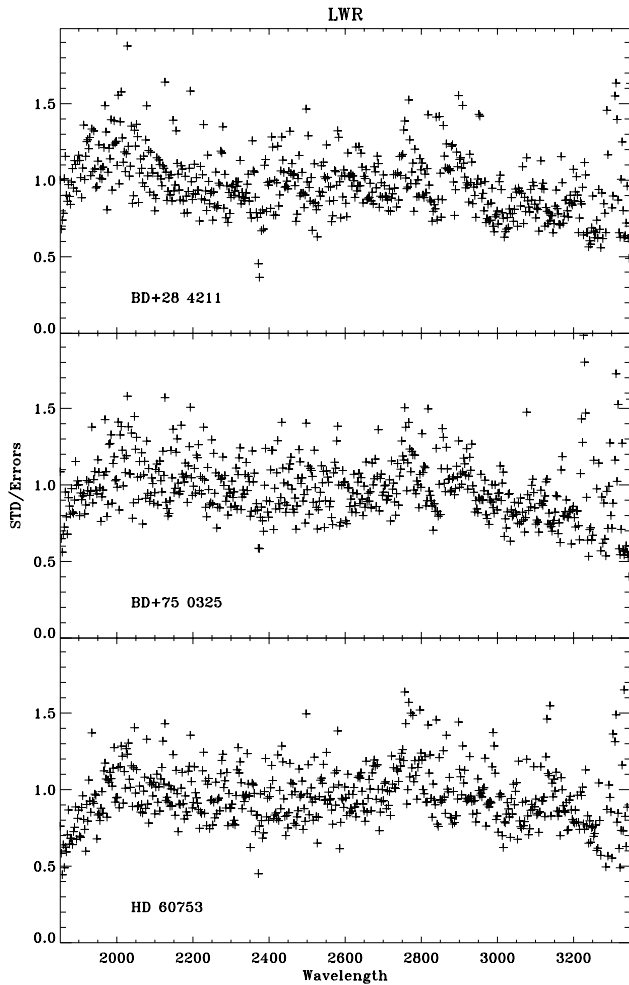
Fig. 17. Same as Fig. 15, but for the LWR camera with a voltage of -5.0 kV
