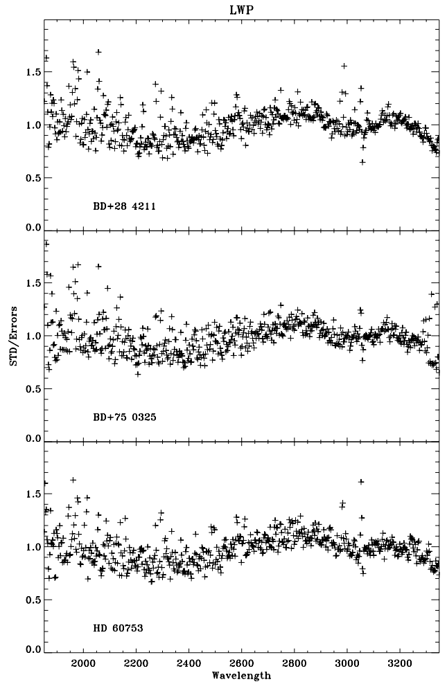
Fig. 16. Same as Fig. 15, but for the LWP camera
