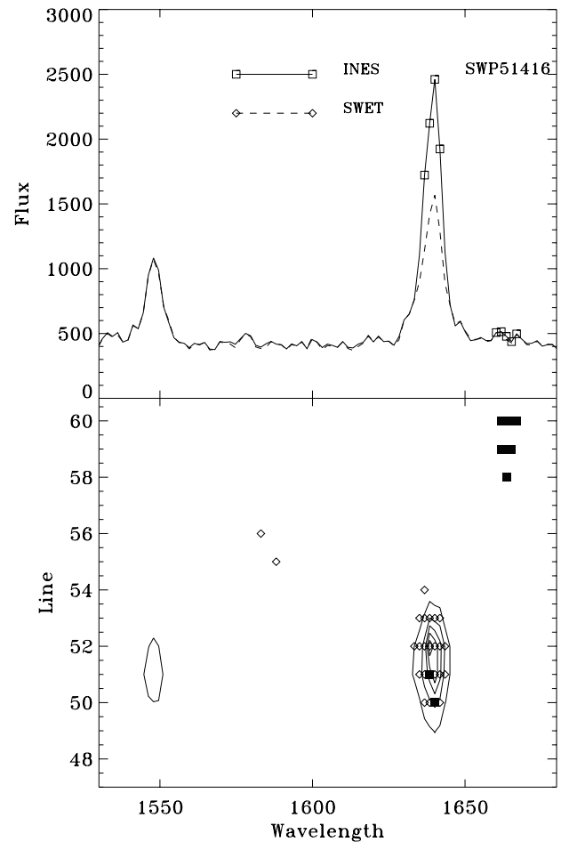
Fig. 9. This figure is similar to Fig. 7, but in this spectrum the HeII line is flagged in the INES spectrum, while it is not in the SWET extraction. As shown in the bottom panel, there are two pixels flagged as saturated in the SILO file. While these flags are propagated to the INES extracted spectrum, they disappear in the SWET extraction. Symbols are as in Fig. 7. In particular, the two solid squares on the HeII line in the SILO file mark saturated pixels
