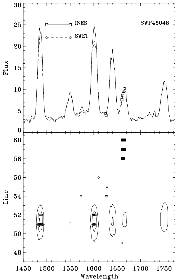
Fig. 8. In this spectrum of Nova V351 Puppis 1991 none of the emission lines are flagged in either of the extractions, but the NIV 1486 Å and the [NeIV] 1602 Å lines have been identified by SWET as “cosmic rays”, and their intensity is underestimated. Symbols are as in Fig. 7
