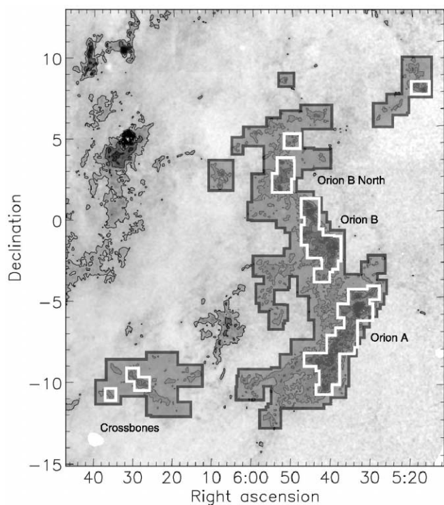
FIG. 3.—Extinction map of Orion, showing the approximate area planned to be mapped with SCUBA-2. The areas surrounded by the dark border will be mapped in the wide, shallow survey, and the areas surrounded by the white border will be mapped in the narrow, deep survey.
