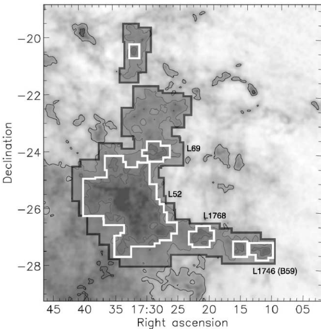
Fig. 10.—Extinction map of the Pipe Nebula. Details as in Fig. 3.
