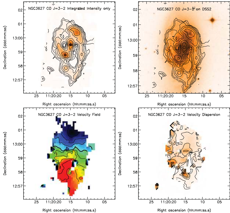
Figure C11. CO J = 3-2 images for NGC 3627. (a) CO J = 3-2 integrated intensity image. Contour levels are (0.5, 1, 2, 4, 8, 16, 32) K km s -1 ( T_{MB} ). (b) CO J = 3-2 overlaid on a Digitized Sky Survey image. (c) Velocity field. Contour levels are (559, 605, 651, 697, 743, 789, 835, 881) km s -1 . (d) The velocity dispersion \sigma_v as traced by the CO J = 3-2 second moment map. Contour levels are (4, 8, 16, 32, 64, 128) km s -1 . Similar images derived from the same data have been published in Warren et al. (2010).
