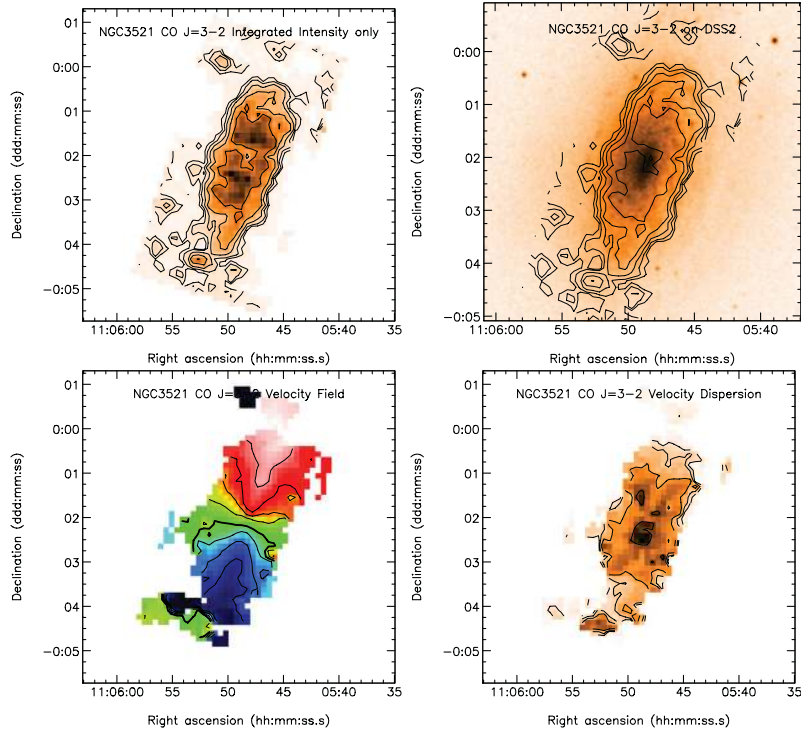
Figure C10. CO J = 3-2 images for NGC 3521. (a) CO J = 3-2 integrated intensity image. Contour levels are (0.5, 1, 2, 4, 8) K km s -1 ( T_{MB} ). (b) CO J = 3-2 overlaid on a Digitized Sky Survey image. (c) Velocity field. Contour levels are (558, 613, 668, 723, 778, 833, 888, 943, 998) km s -1 . (d) The velocity dispersion \sigma_v as traced by the CO J = 3-2 second moment map. Contour levels are (4, 8, 16, 32) km s -1 . Similar images derived from the same data have been published in Warren et al. (2010).
