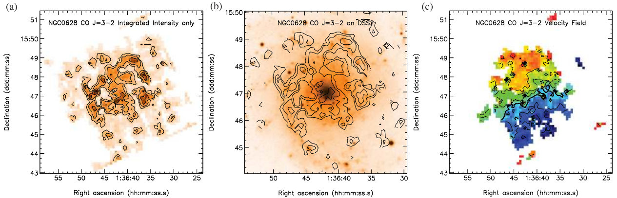
Figure C1. CO J = 3-2 images for NGC 0628. (a) CO J = 3-2 integrated intensity image. Contours levels are (0.5, 1, 2) K km s ^{-1} ( T_{\text{MB}} ). (b) CO J = 3-2 integrated intensity contours overlaid on an optical image from the Digitized Sky Survey. (c) Velocity field as traced by the CO J = 3-2 first moment map. Contour levels are (624, 632, 640, 648, 656, 664, 672, 680) km s ^{-1} . The thick line shows the systemic velocity given in Table 1. Similar images derived from the same data have been published in Warren et al. (2010). The velocity dispersion map has been published in Wilson et al. (2011).
