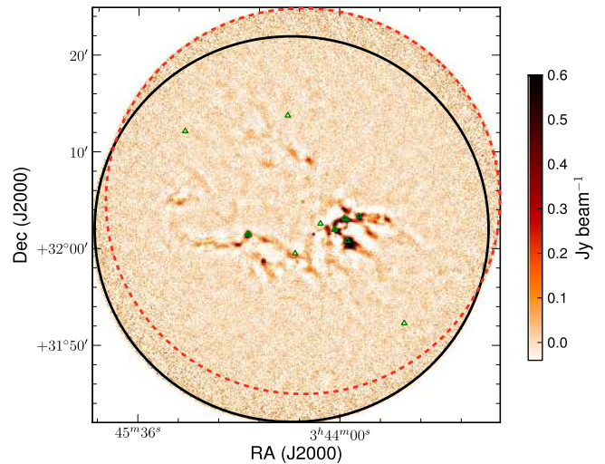
Figure 10. The Transient Survey field IC 348 mosaicked with its corresponding archival GBS fields at 850 \mu\text{m} . The area of each observed GBS and Transient Survey field included in the mosaic is bounded by a circle. The solid black circle is the Transient Survey field. The red (dashed) circle shows the boundary of the IC 348-E GBS field. The green triangles represent the positions of known protostars taken from the Spitzer Space Telescope catalog of Dunham et al. (2015).
