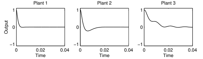
Figure 5 System responses of the original continuous-time control loops.
