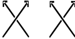
FIGURE 4. positive and negative crossings, respectively.
