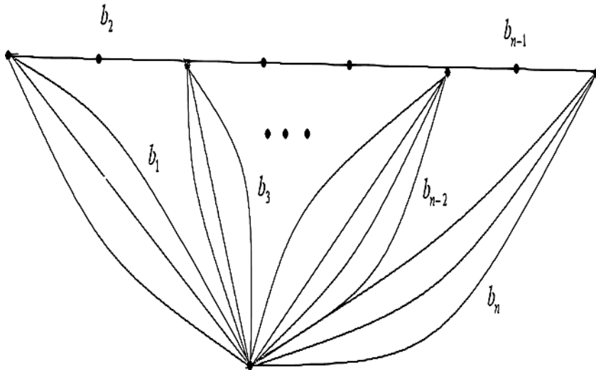
FIGURE 3. The canonical Tait graph associated to the sequence \{b_1, \dots, b_n\} of positive integers with an odd integer n = 2k + 1 .
