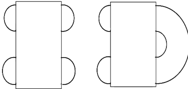
FIGURE 1. The closure of the 4-braid according to whether the last element of the product is \sigma_2^{\pm 1} or \sigma_1^{\pm 1} , respectively.
