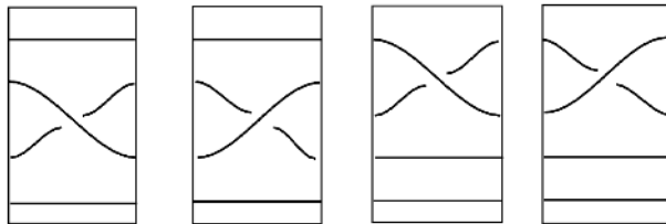
FIGURE 2. The 4-braids \sigma_2, \sigma_2^{-1}, \sigma_1, and \sigma_1^{-1} , respectively.
