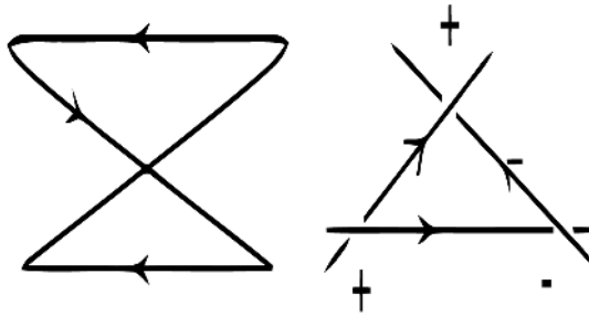
FIGURE 5. The case where \sigma_D = (23) and one of the cases of \varepsilon_i .
