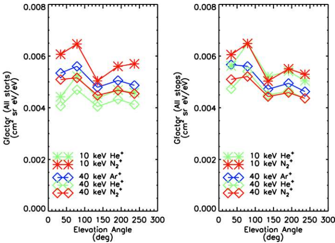
Fig. 65 Geometric factor measured during calibration includes detector efficiency. The dip seen at 135° is where the ion beam is incident at an angle between two anodes and mechanical structures in the instrument partially obscure the beam
