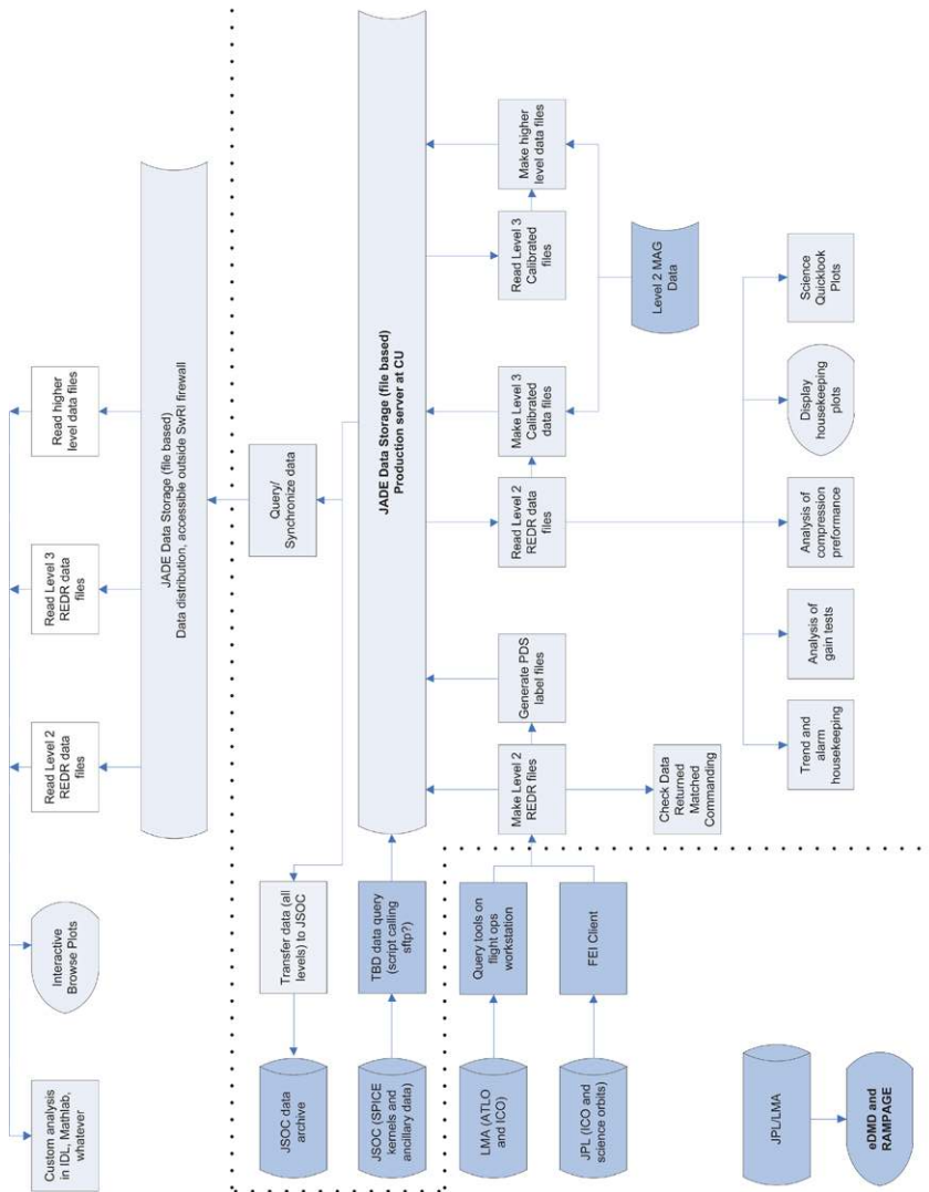
Fig. 78 Data processing pipeline flow
