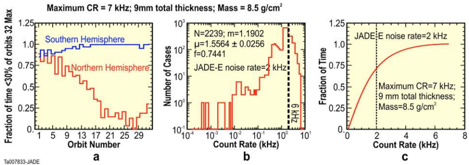
Fig. 44 Similar to Fig. 43, but for JADE-E and using a 9-mm thick shield with a stopping power of 8.5 g/cm 2
