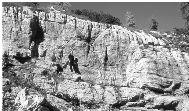
Fig. 8 Lower Member of the Prehodavci Formation: light gray nodular limestone. Triglav Lakes Valley, section TV2
