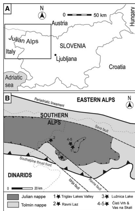
Fig. 1 a Location of the Julian Alps. Inset in a represents the location of b. b Main structural elements in NW Slovenia and location of the investigated sections
