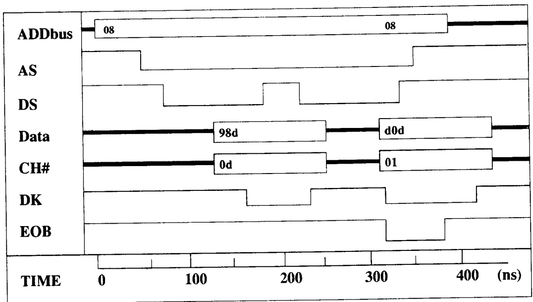
Fig. 4.3. Transfer cycle.
