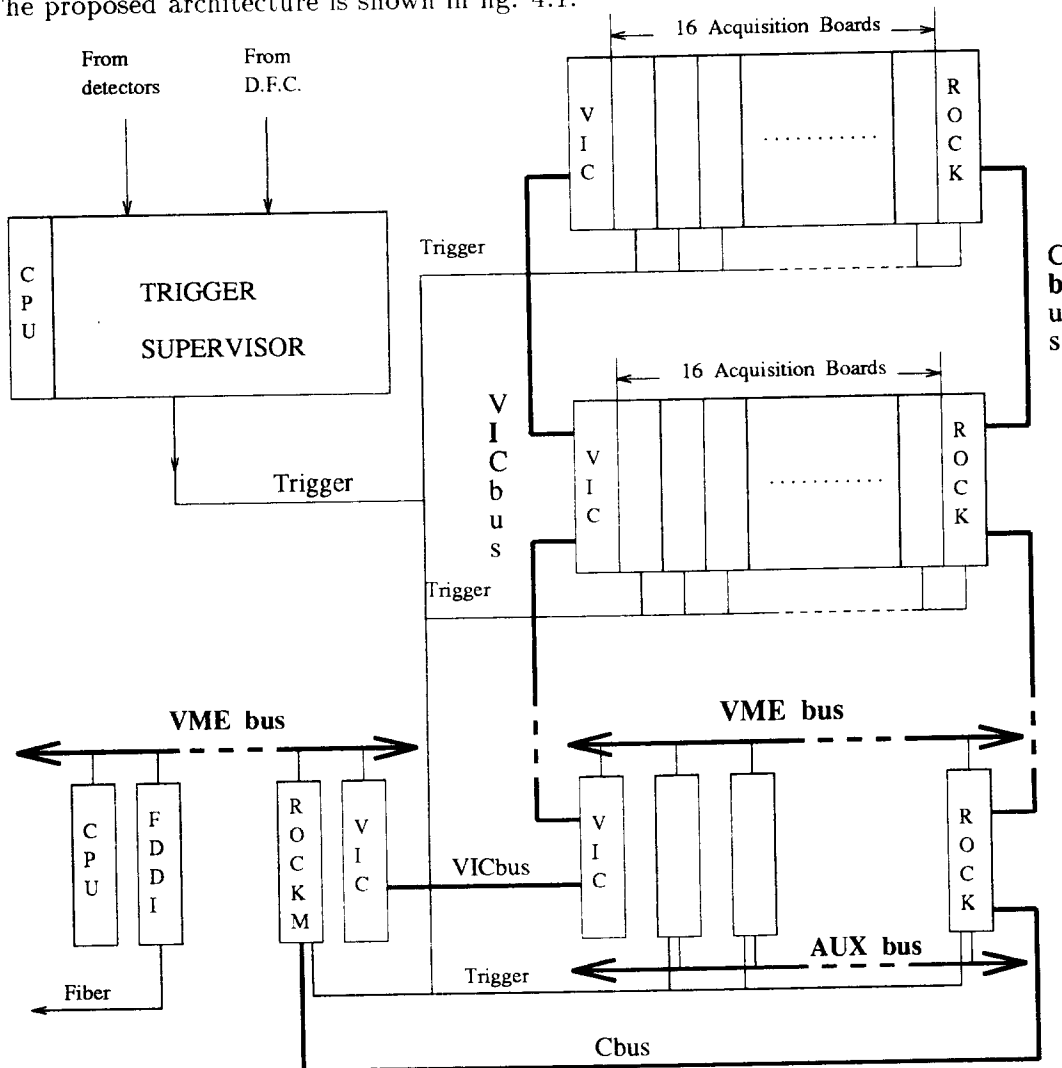
Fig. 4.1. System Architecture.
