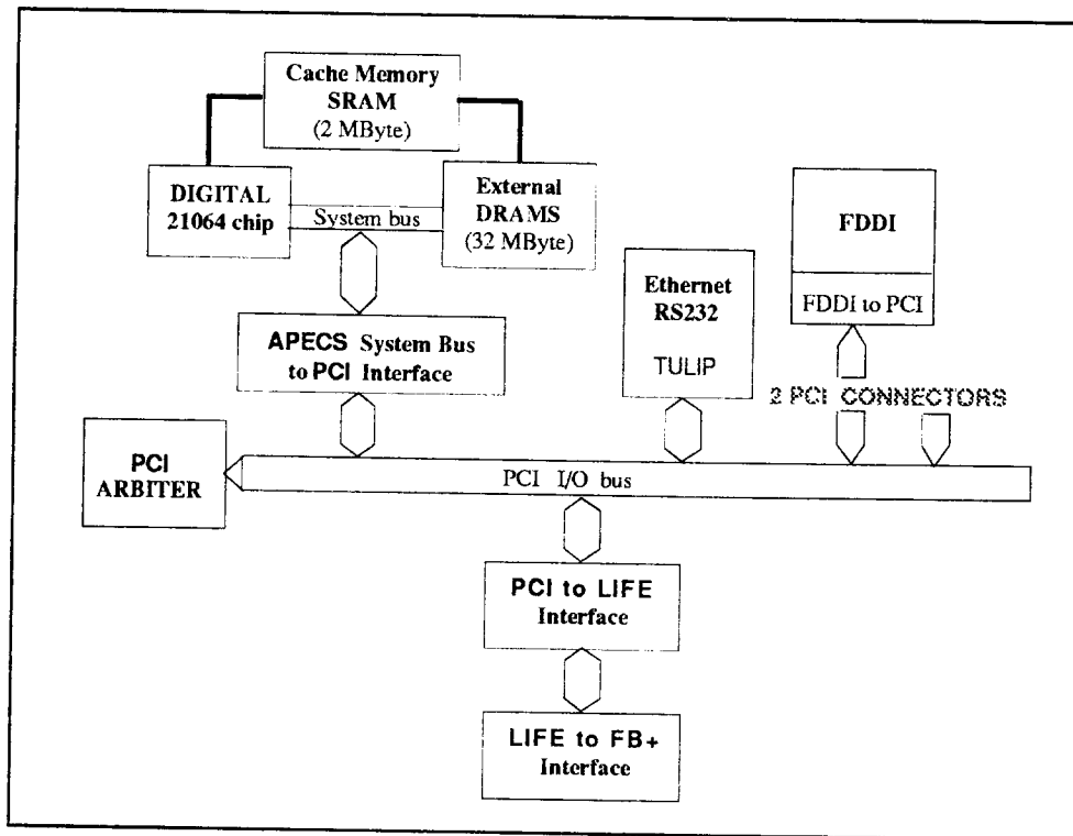
Fig. 6.1. SBC+ architecture.
