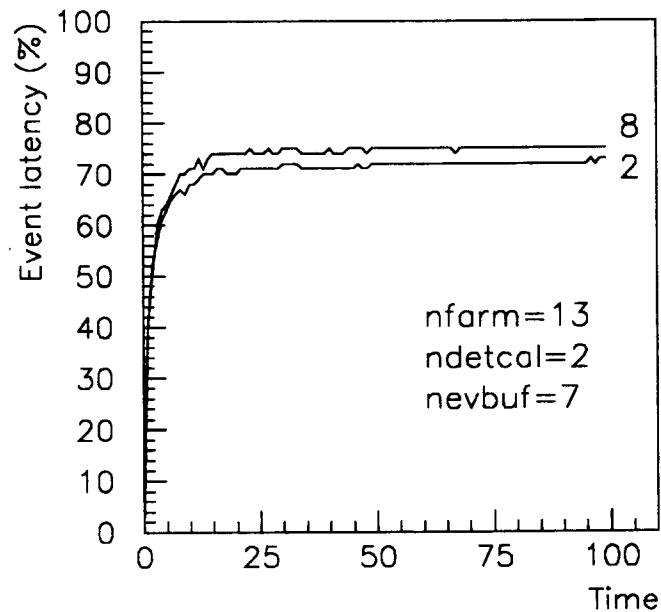
Fig. 5.6. Event latency.
