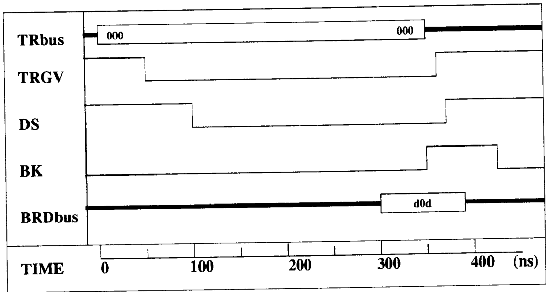
Fig. 4.2. Broadcast cycle.
