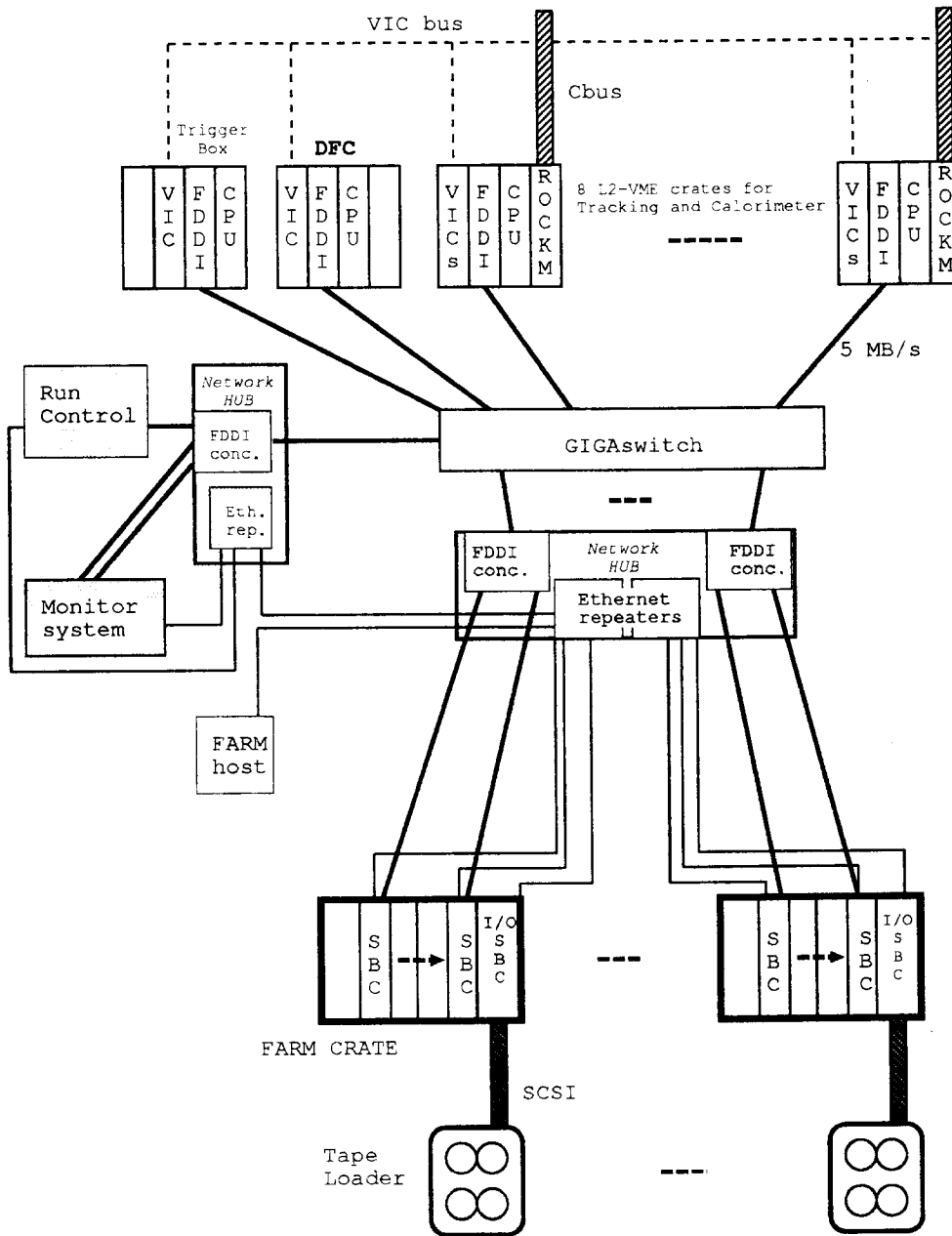
Fig. 5.2. DAQ system architecture.
