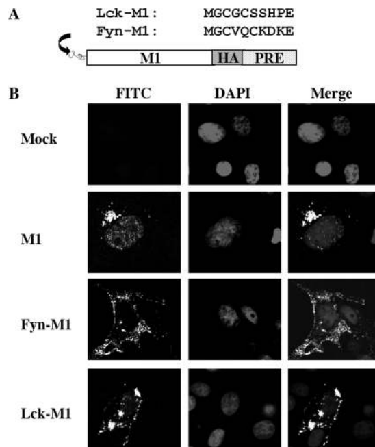
FIG. 3. Membrane targeting domains redirect M1 to the plasma membrane. (A) Schematic representation of two membrane targeting domains derived from Fyn and Lck oncoproteins that were appended to the M1 N terminus. (B) Representative M1 subcellular localization images in COS-1 cells expressing M1 or Fyn-M1 or Lck-M1. At 48 h posttransfection, COS-1 cells individually transfected with pM1, pFyn-M1, pLck-M1, and empty vector (mock) were fixed, permeabilized, and stained with goat anti-M1 IgG-FITC. Nuclei of COS-1 cells were stained with DAPI. M1 localization among these cells was then examined by confocal microscopy at an \times 60 magnification.
