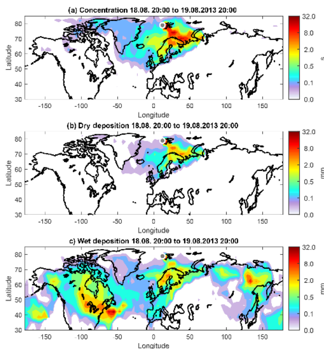
Figure 3. Source–receptor relationships (for emissions occurring in the lowest 100 m a.g.l.) for black carbon observed at Ny-Ålesund in Svalbard for a 24 h period starting on 18 August 2013 at 20:00 UTC. The sensitivities were calculated for (a) concentrations ( s ) in the layer 0–100 m a.g.l., (b) dry deposition (mm) and (c) wet deposition (mm).
