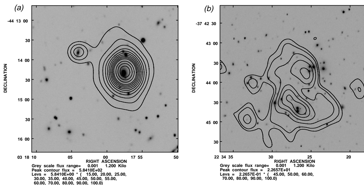
Figure 3 —(a) Abell 3112 and (b) Abell 3888. The grey scale is an R -band optical image of the cluster core taken at LCO. The overlaid contours represent the ROSAT HRI X-ray images which show the gas distribution within each of the clusters.
