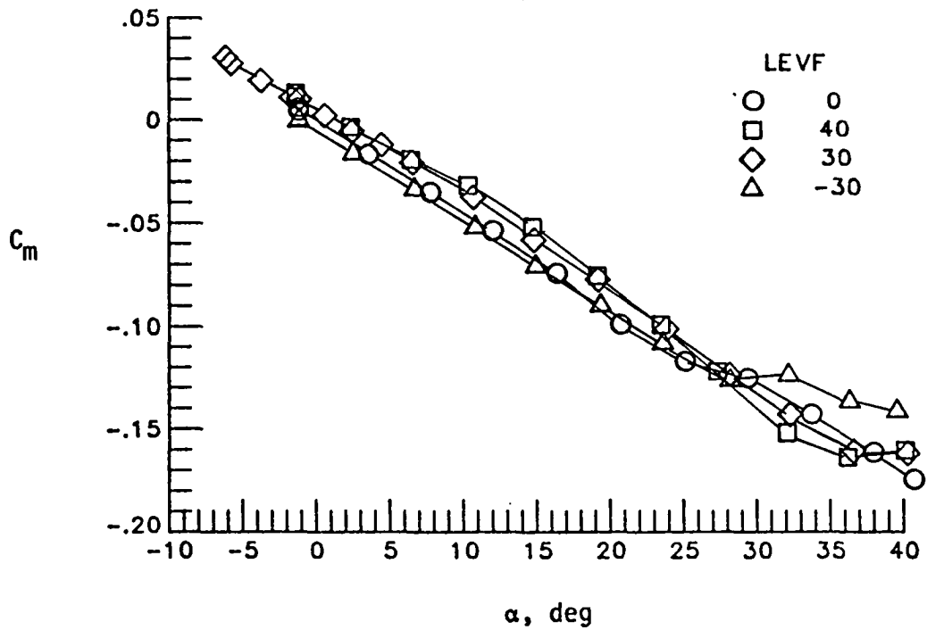
(b) Pitching moment characteristics.
