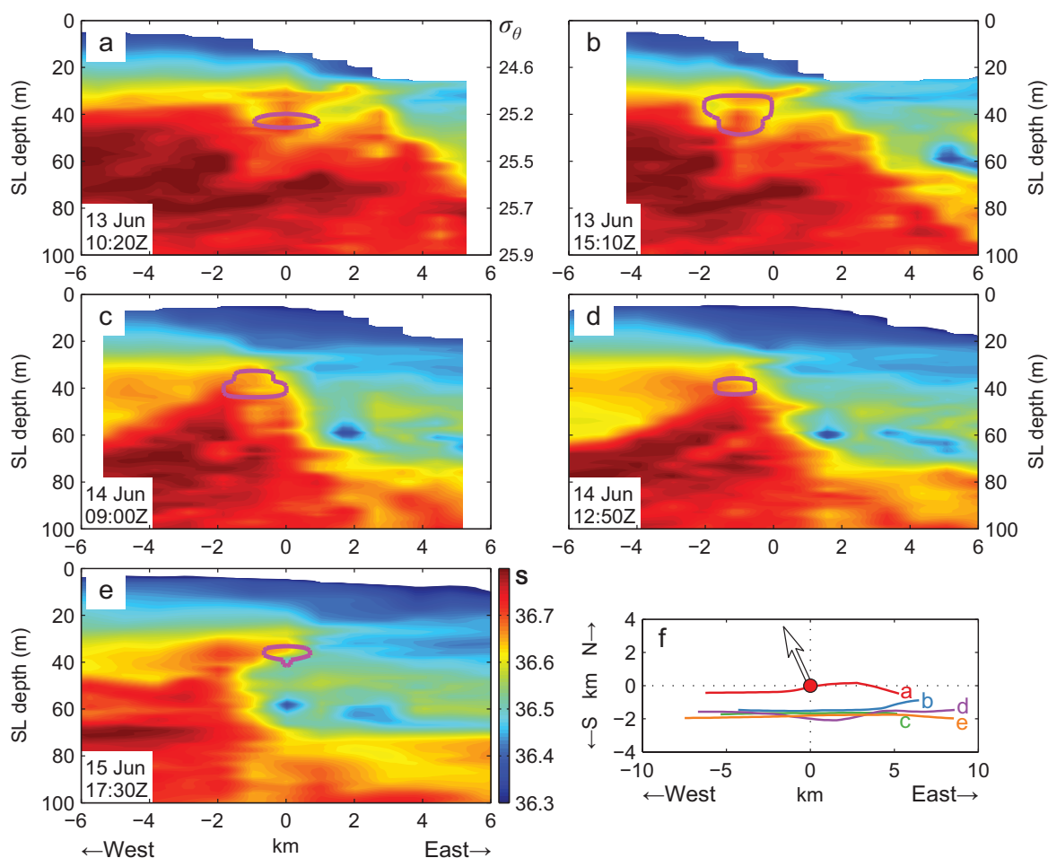
FIG. 10. (a)–(e) High-resolution zonal MVP sections showing evolution of a north–south-oriented thermo-haline (spice) front in the vicinity of the rhodamine dye patch between 13 and 15 Jun 2011 under a \sim 0.1\text{f} confluence. The vertical axis is an isopycnal (semi-Lagrangian) depth: namely, the average depth of an isopycnal, and corresponding potential density values are marked on the right in (a). The magenta contour shows evolution of the rhodamine dye patch. (f) Location of sections shown in (a)–(e) in the advected frame of reference moving with the center of mass of the drifter array (red circle). The arrow shows the mean advection direction during the 13–15 Jun period.
