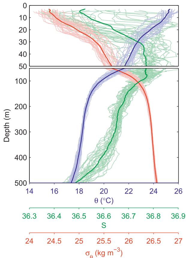
FIG. 1. Profiles of potential temperature (blue), salinity (green), and potential density (red) during LatMix Seaglider deployment (3–10 Jun 2011). Heavy lines indicate the mean profiles. Salinity is reported on the practical salinity scale throughout (nondimensional).
