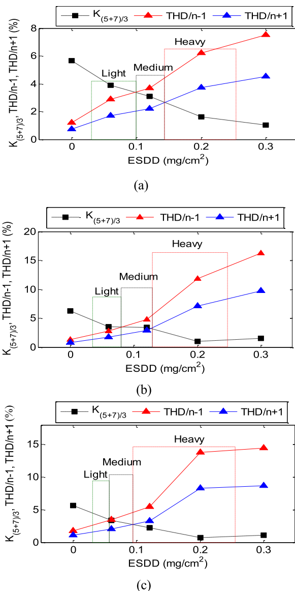
FIGURE 14. K_{(5+7)/3} , THD/n-1 and THD/n+1 for insulator string A (SA) at: (a) 7 \pm 0.5 \text{ g/s.cm}^3 , (b) 43.3 \pm 1.5\text{g/s.cm}^3 , (c) 83.8 \pm 2.3 \text{ g/s.cm}^3 .
