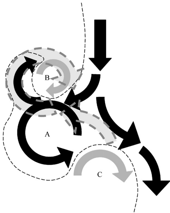
Fig. 3. Schematic of formation of eddy pairs in the Leeuwin Current and Undercurrent. The black arrows represent the Leeuwin Current heading southward along the coast and the thin dashed line represents the warm water boundary. The solid grey arrows represent cooler offshore water and the grey dashed arrows represent the Leeuwin Undercurrent. (A) Leeuwin Current anticyclonic eddy. (B) Undercurrent cyclonic eddy which at the surface appears as a cyclonic eddy enclosing oceanic water, and paired with surface LC eddy. (C) New eddy forming from ocean water drawn between the Leeuwin Current and the anticyclonic eddy. Figure from Rennie et al. (2007) with permission.
