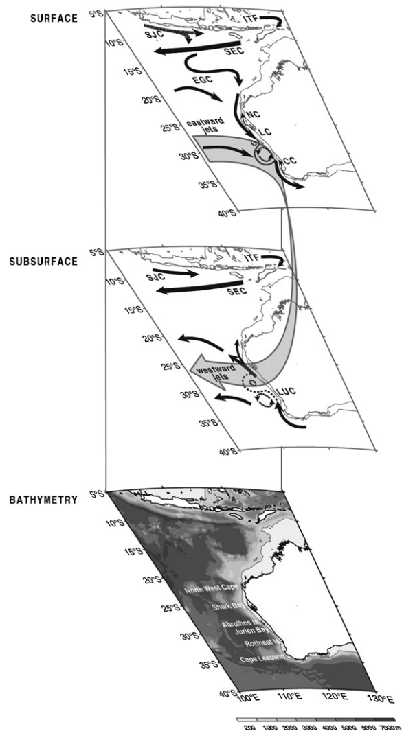
Fig. 1. Simplified schematic of surface currents off Western Australia emphasizing the connection between the Leeuwin Current (LC) and Leeuwin Undercurrent (LUC) as a curved vertical arrow. Indicated is (1) the bathymetry and key coastal landmarks (bottom), (2) the subsurface (200–400 m) northward-flowing LUC, showing westward jets offshore, (3) the LC at the surface, fed by the eastward jets transporting Subtropical Water / South Indian Central Water into the LC and then the LUC. The relative position of other regional currents is referred to in the text. Papers in this volume address key questions regarding the origin of the Leeuwin Current from both the Indonesian Throughflow (ITF) and the South Java Current (SJC) and its interaction with adjacent water masses including the wind-driven counter-currents, the Capes Current (CC) and the Ningaloo Current (NC). Thanks to Sue Wijffels (CSIRO, Hobart) for helpful discussions on this figure.
