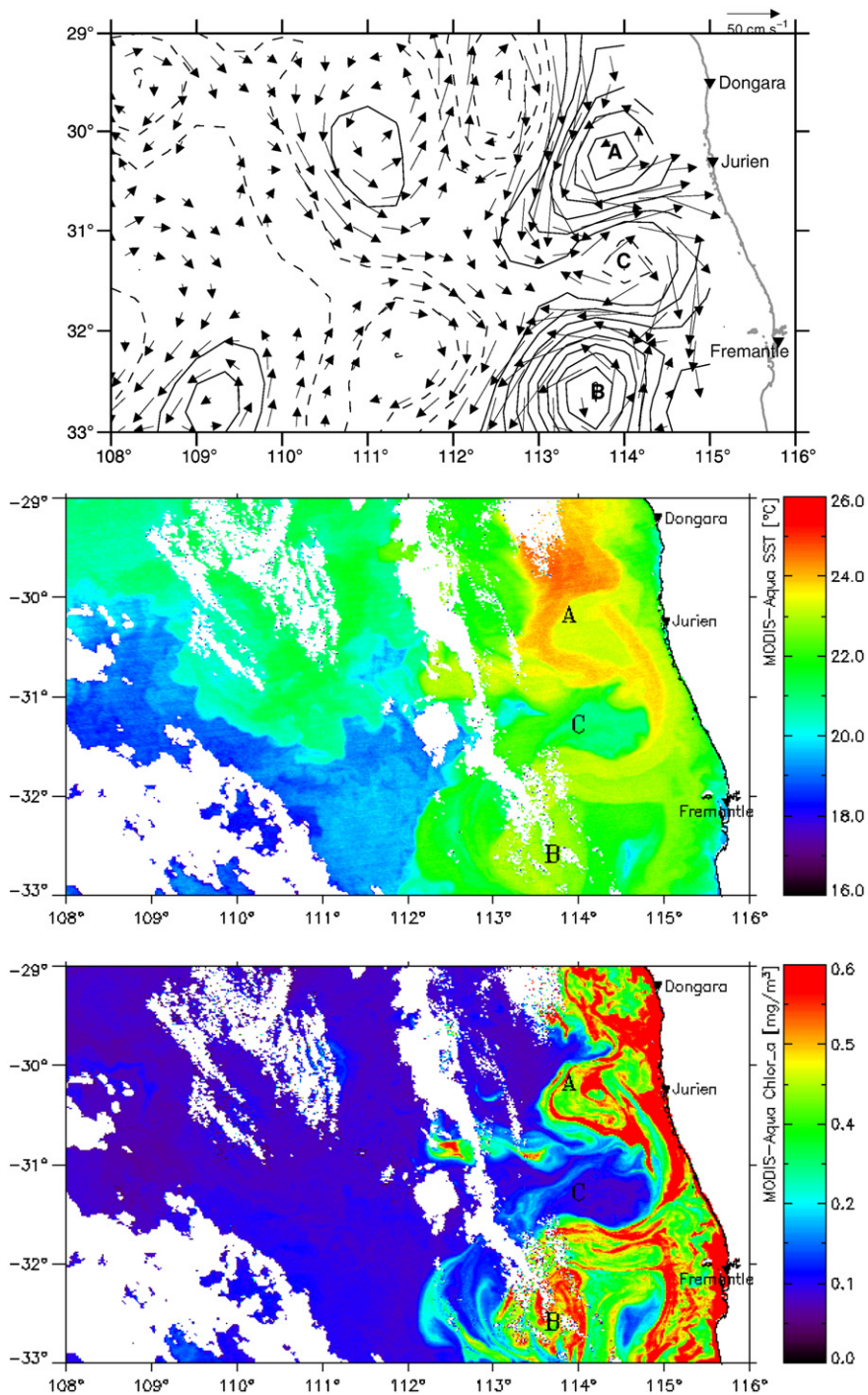
Fig. 2. Typical structure of forming LC eddies. (a) Sea surface height anomaly and surface geostrophic current anomaly (arrows) in the southeast Indian Ocean on 28 May 2003. (b) SST and (c) SSC concentration from MODIS satellite in the same region as (a) on 25 May 2003. Note the formation of a WC-CC-WC triplet. Figure from Feng et al. (2007) with permission.
