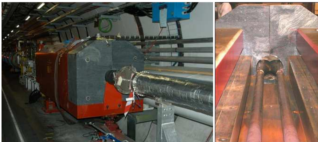
Figure 1.3: Photo of the TAN absorber located 140 m from the IP. Left: TAN fully assembled in the LHC tunnel seen from the IP side. Right: TAN during assembly at CERN seen from the top facing the IP. The 96 mm gap between the two beam pipes allows space for installation of detectors.
