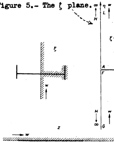
Figure 4.- Conformal transformation of the \zeta on the Z plane.
