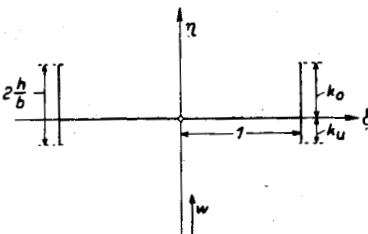
Figure 2.- Section through vortex surface leaving the wing with end plates.
