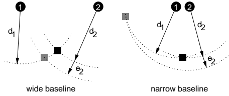
Figure 1: Errors in estimated node location depend on whether or not the points of reference for multilateration form a wide baseline.
